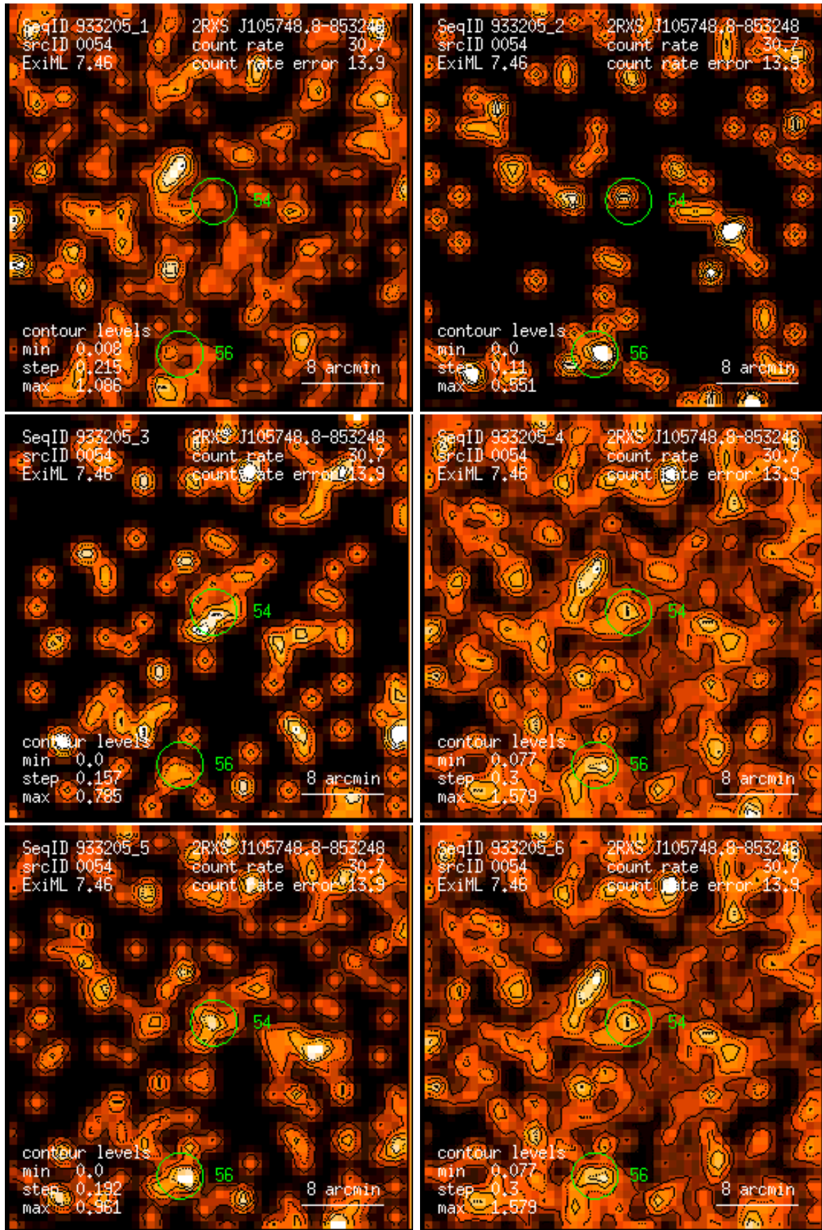
Figure 54: RASS 933205: detection 0054: band rate images, Gaussian filter: (1) PSPC channels 11 – 41, (2) 52 – 90, (3) 91 – 201, (4) 11 – 235, (5) 52 – 201, (6) 11 – 201. Broad band rates in counts/ks. Band rate contour levels in counts/ks/arcmin 2 .
