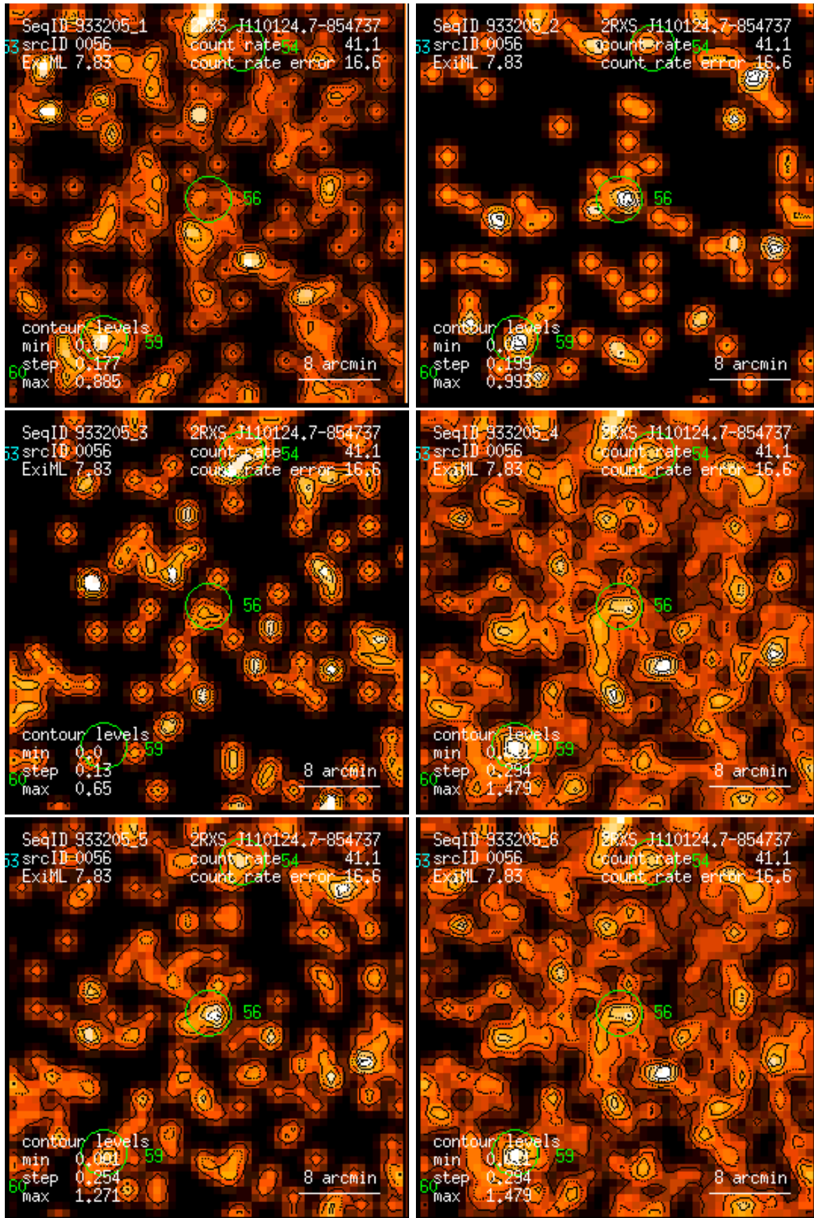
Figure 56: RASS 933205: detection 0056: band rate images, Gaussian filter: (1) PSPC channels 11 – 41, (2) 52 – 90, (3) 91 – 201, (4) 11 – 235, (5) 52 – 201, (6) 11 – 201. Broad band rates in counts/ks. Band rate contour levels in counts/ks/arcmin 2 .
