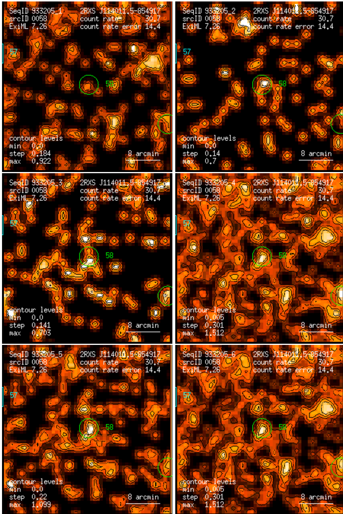
Figure 58: RASS 933205: detection 0058: band rate images, Gaussian filter: (1) PSPC channels 11 – 41, (2) 52 – 90, (3) 91 – 201, (4) 11 – 235, (5) 52 – 201, (6) 11 – 201. Broad band rates in counts/ks. Band rate contour levels in counts/ks/arcmin 2 .
