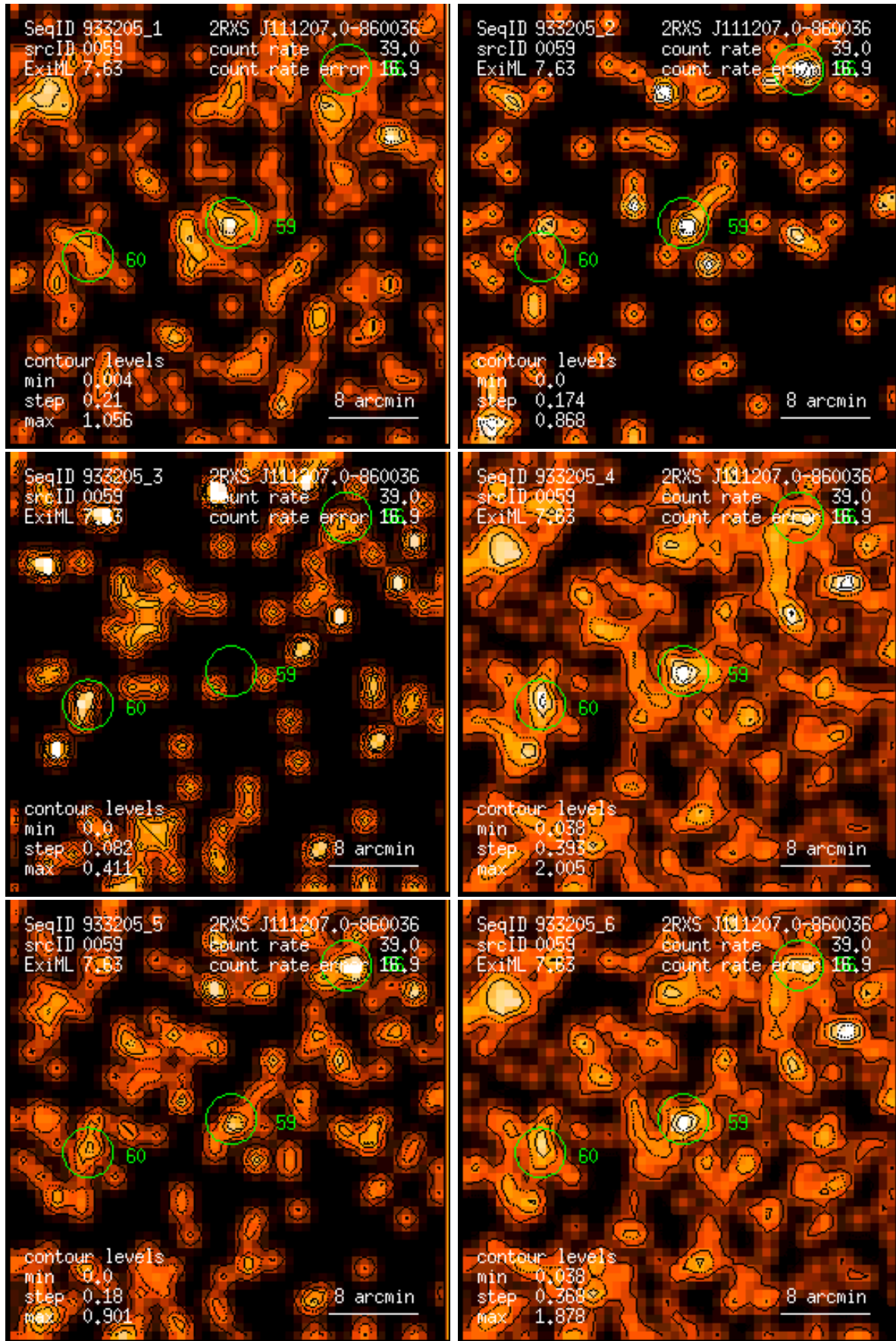
Figure 59: RASS 933205: detection 0059: band rate images, Gaussian filter: (1) PSPC channels 11 – 41, (2) 52 – 90, (3) 91 – 201, (4) 11 – 235, (5) 52 – 201, (6) 11 – 201. Broad band rates in counts/ks. Band rate contour levels in counts/ks/arcmin 2 .
