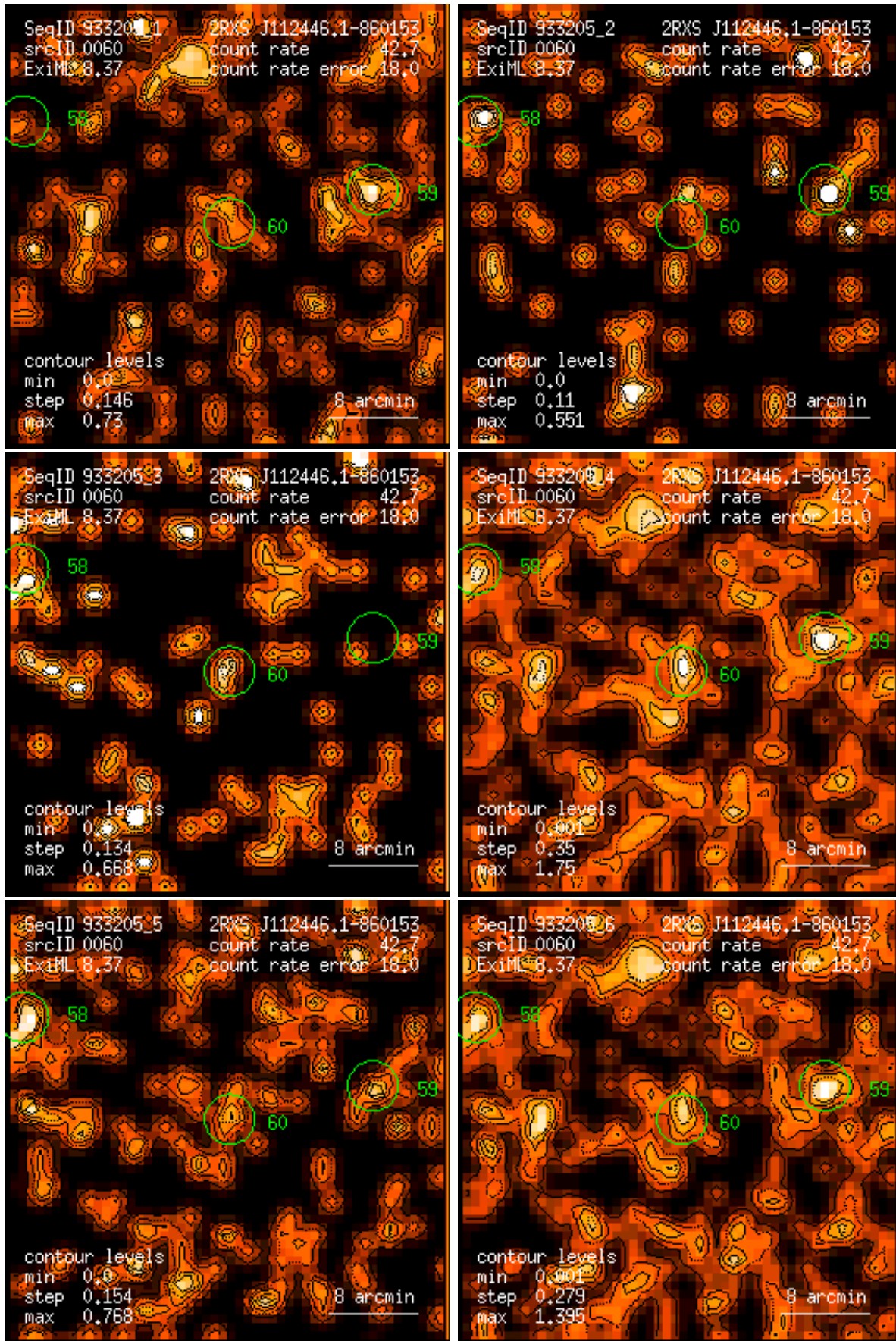
Figure 60: RASS 933205: detection 0060: band rate images, Gaussian filter: (1) PSPC channels 11 – 41, (2) 52 – 90, (3) 91 – 201, (4) 11 – 235, (5) 52 – 201, (6) 11 – 201. Broad band rates in counts/ks. Band rate contour levels in counts/ks/arcmin 2 .
