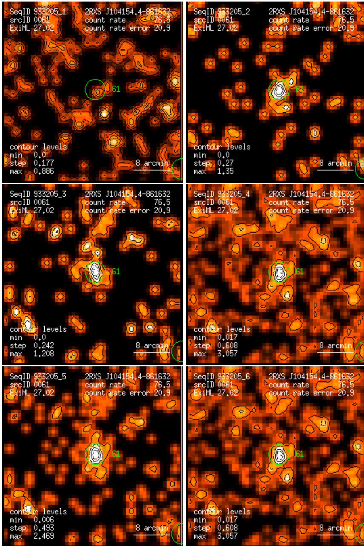
Figure 61: RASS 933205: detection 0061: band rate images, Gaussian filter: (1) PSPC channels 11 – 41, (2) 52 – 90, (3) 91 – 201, (4) 11 – 235, (5) 52 – 201, (6) 11 – 201. Broad band rates in counts/ks. Band rate contour levels in counts/ks/arcmin 2 .
