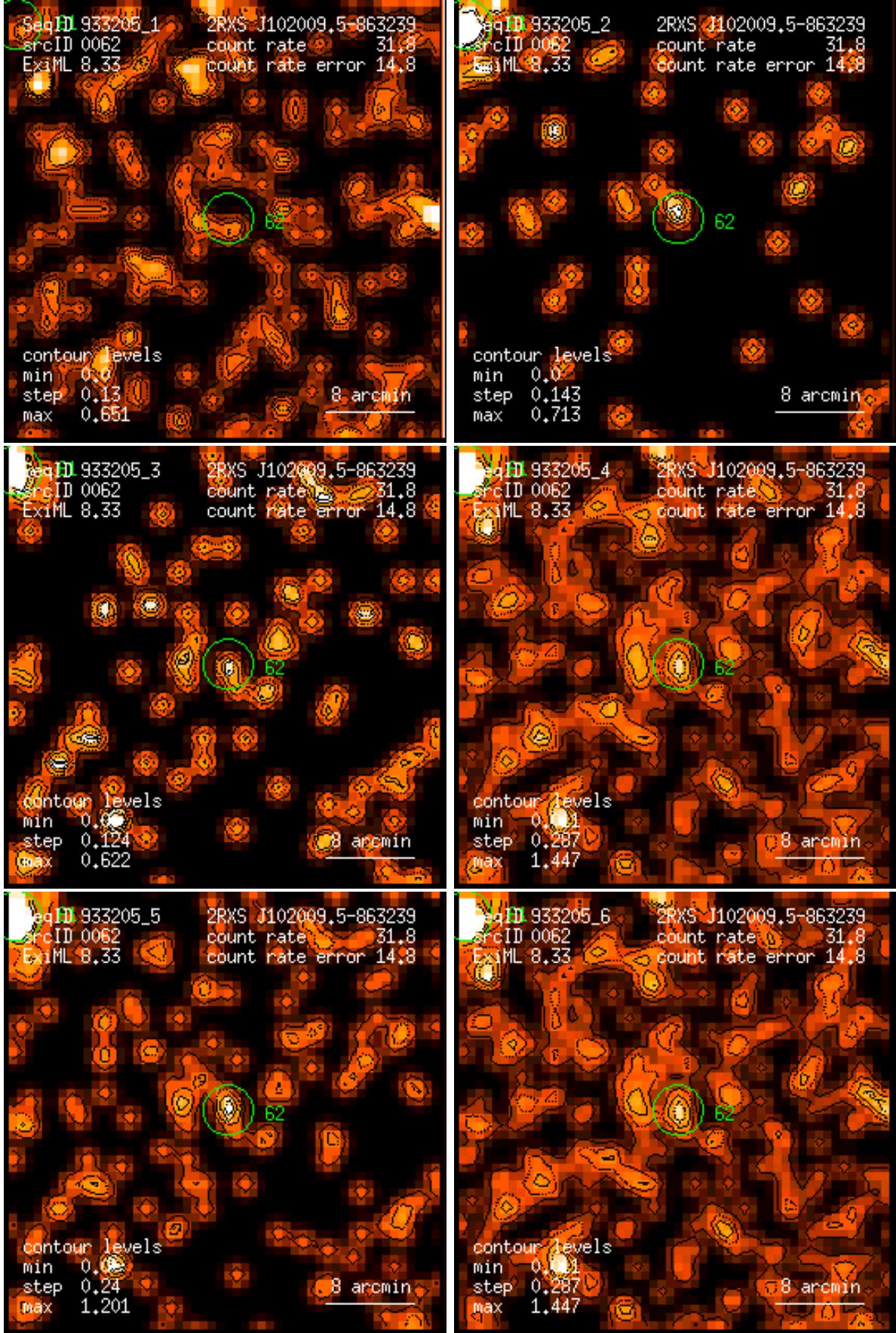
Figure 62: RASS 933205: detection 0062: band rate images, Gaussian filter: (1) PSPC channels 11 – 41, (2) 52 – 90, (3) 91 – 201, (4) 11 – 235, (5) 52 – 201, (6) 11 – 201. Broad band rates in counts/ks. Band rate contour levels in counts/ks/arcmin 2 .
