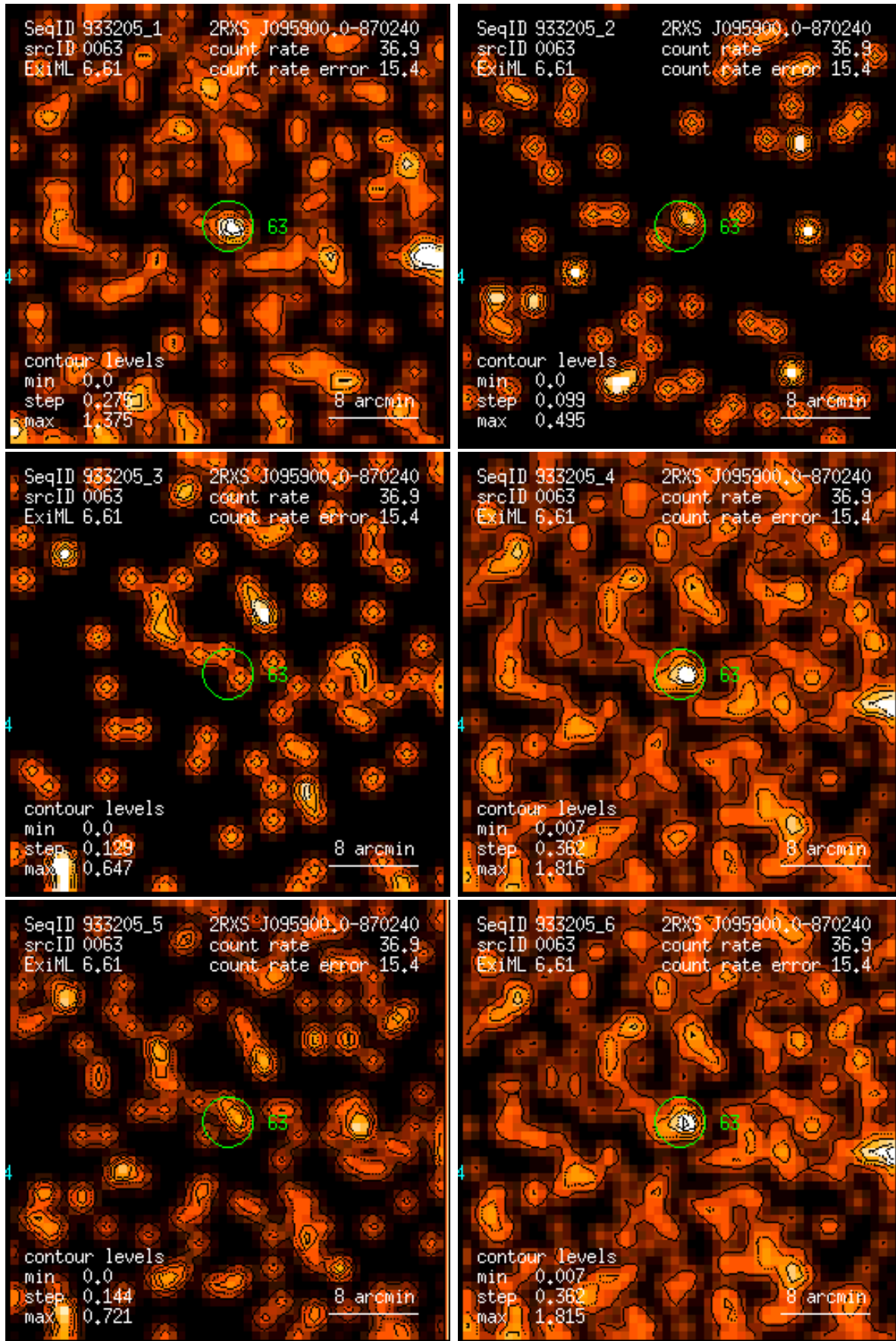
Figure 63: RASS 933205: detection 0063: band rate images, Gaussian filter: (1) PSPC channels 11 – 41, (2) 52 – 90, (3) 91 – 201, (4) 11 – 235, (5) 52 – 201, (6) 11 – 201. Broad band rates in counts/ks. Band rate contour levels in counts/ks/arcmin 2 .
