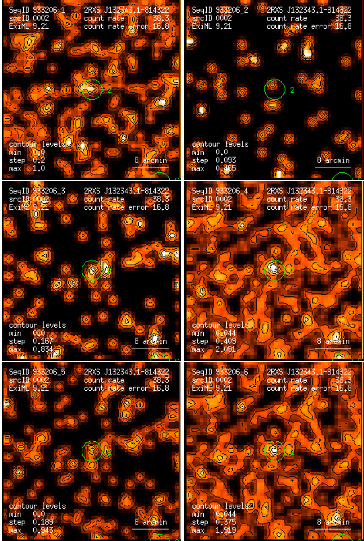
Figure 2: RASS 933206: detection 0002: band rate images, Gaussian filter: (1) PSPC channels 11 – 41, (2) 52 – 90, (3) 91 – 201, (4) 11 – 235, (5) 52 – 201, (6) 11 – 201. Broad band rates in counts/ks. Band rate contour levels in counts/ks/arcmin 2 .
