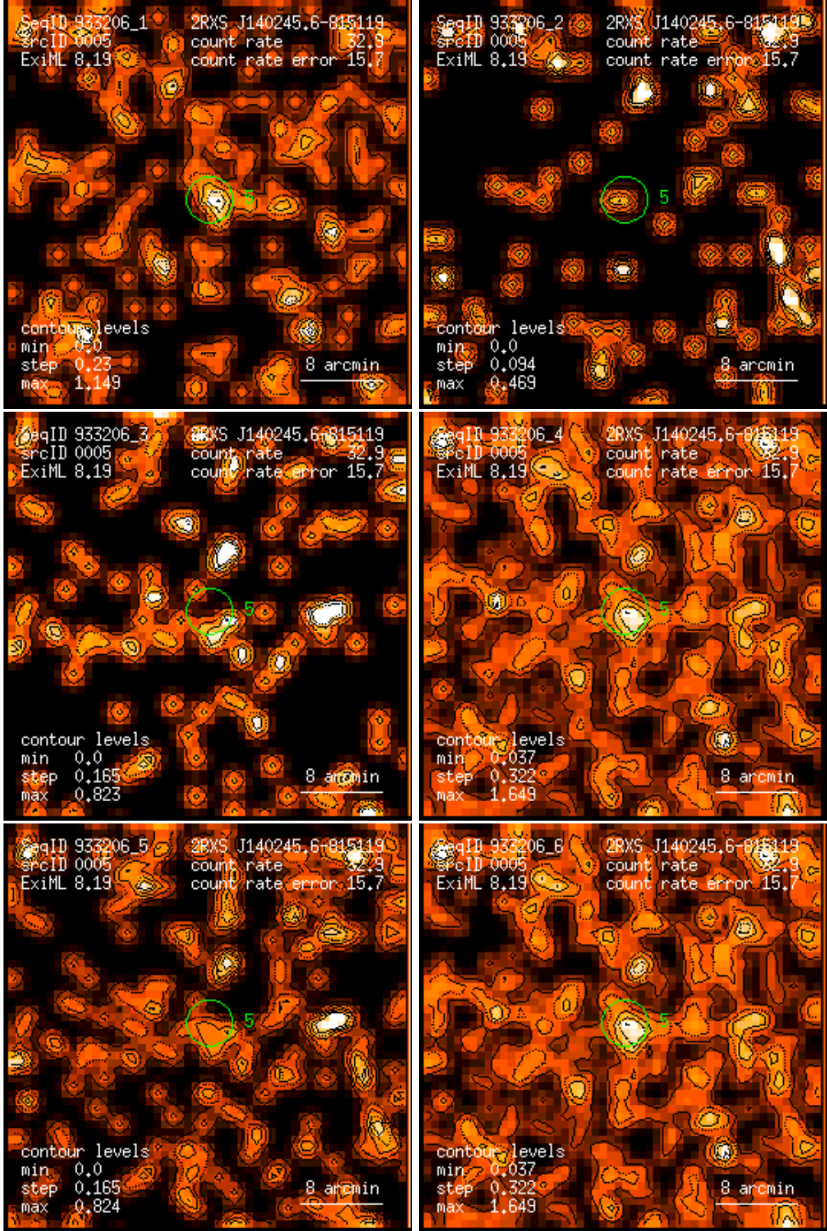
Figure 5: RASS 933206: detection 0005: band rate images, Gaussian filter: (1) PSPC channels 11 – 41, (2) 52 – 90, (3) 91 – 201, (4) 11 – 235, (5) 52 – 201, (6) 11 – 201. Broad band rates in counts/ks. Band rate contour levels in counts/ks/arcmin 2 .
