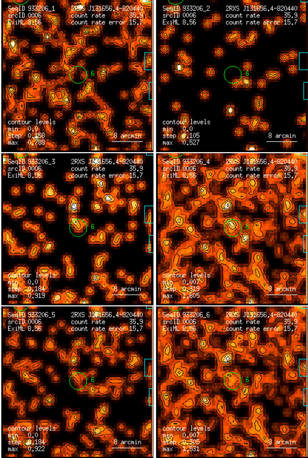
Figure 6: RASS 933206: detection 0006: band rate images, Gaussian filter: (1) PSPC channels 11 – 41, (2) 52 – 90, (3) 91 – 201, (4) 11 – 235, (5) 52 – 201, (6) 11 – 201. Broad band rates in counts/ks. Band rate contour levels in counts/ks/arcmin 2 .
