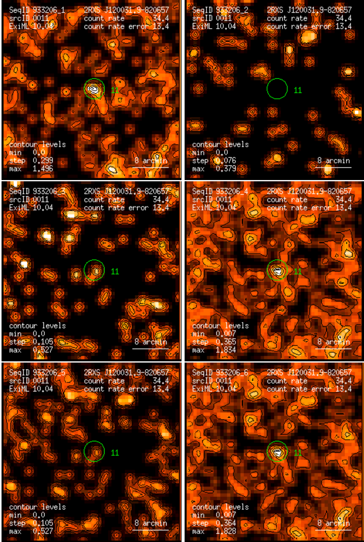
Figure 11: RASS 933206: detection 0011: band rate images, Gaussian filter: (1) PSPC channels 11 – 41, (2) 52 – 90, (3) 91 – 201, (4) 11 – 235, (5) 52 – 201, (6) 11 – 201. Broad band rates in counts/ks. Band rate contour levels in counts/ks/arcmin 2 .
