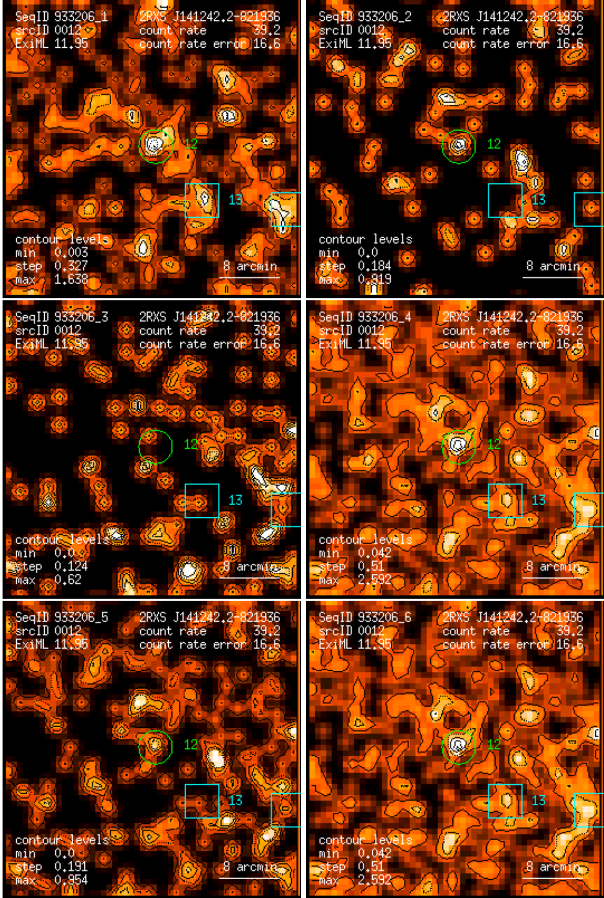
Figure 12: RASS 933206: detection 0012: band rate images, Gaussian filter: (1) PSPC channels 11 – 41, (2) 52 – 90, (3) 91 – 201, (4) 11 – 235, (5) 52 – 201, (6) 11 – 201. Broad band rates in counts/ks. Band rate contour levels in counts/ks/arcmin 2 .
