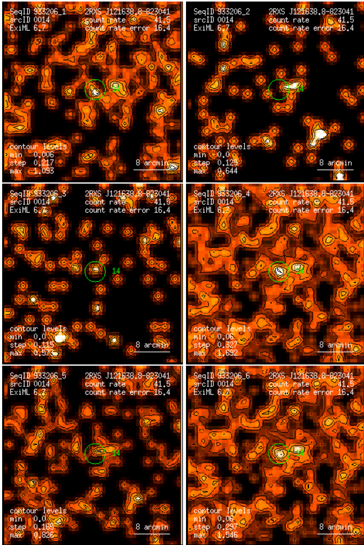
Figure 14: RASS 933206: detection 0014: band rate images, Gaussian filter: (1) PSPC channels 11 – 41, (2) 52 – 90, (3) 91 – 201, (4) 11 – 235, (5) 52 – 201, (6) 11 – 201. Broad band rates in counts/ks. Band rate contour levels in counts/ks/arcmin 2 .
