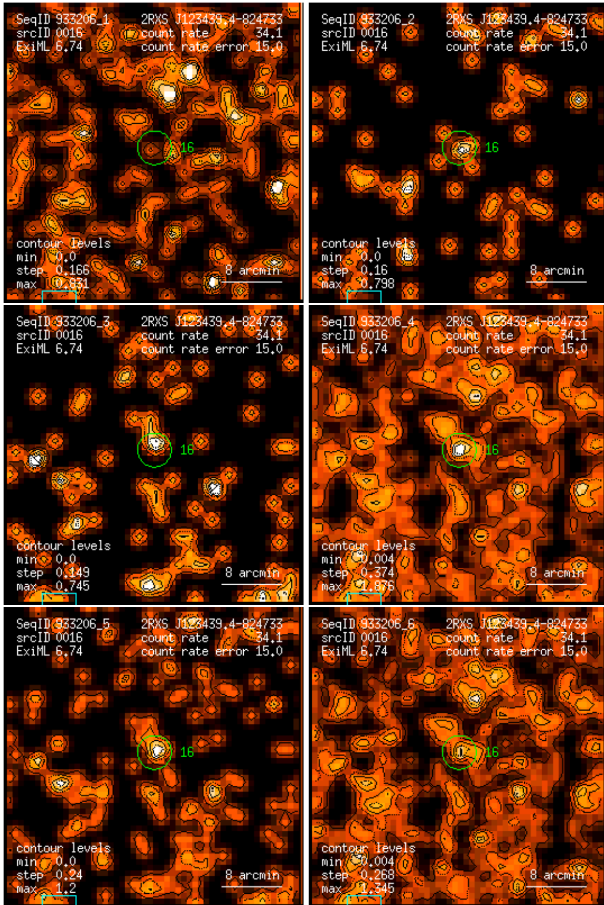
Figure 16: RASS 933206: detection 0016: band rate images, Gaussian filter: (1) PSPC channels 11 – 41, (2) 52 – 90, (3) 91 – 201, (4) 11 – 235, (5) 52 – 201, (6) 11 – 201. Broad band rates in counts/ks. Band rate contour levels in counts/ks/arcmin 2 .
