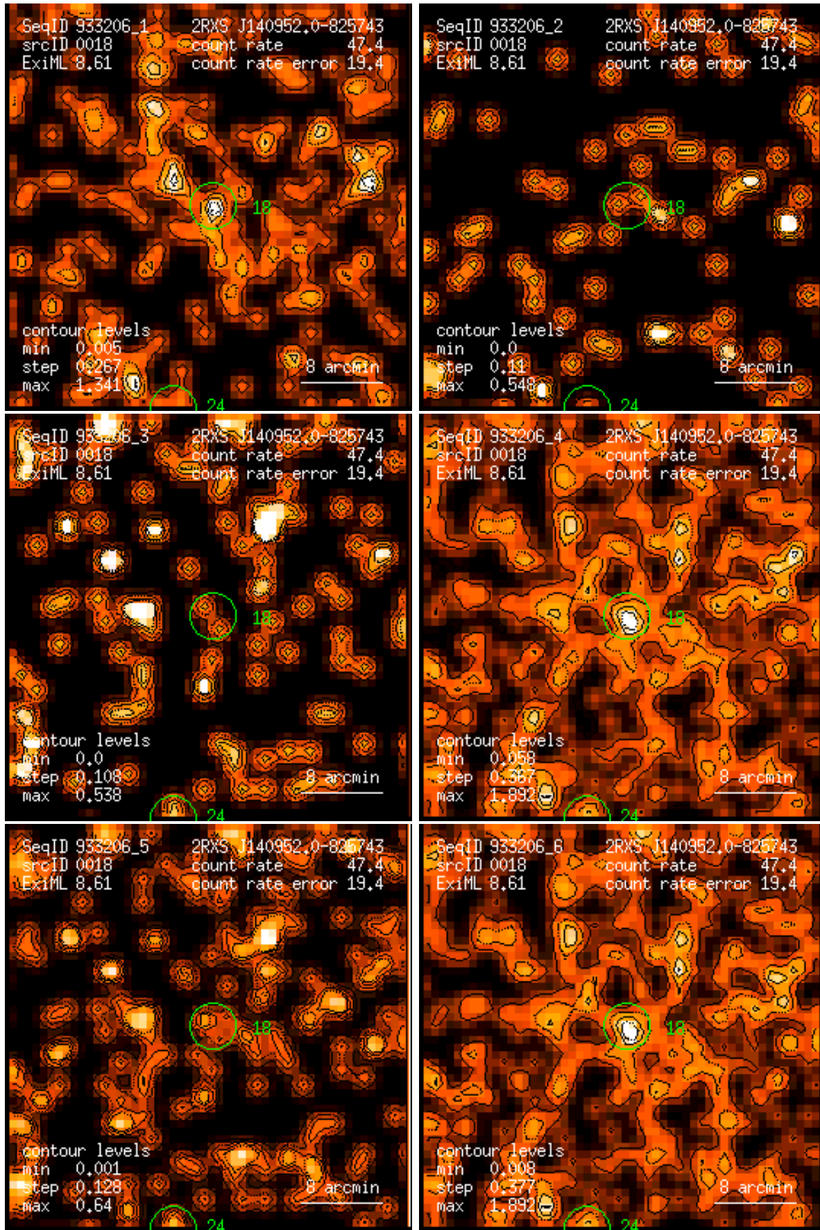
Figure 18: RASS 933206: detection 0018: band rate images, Gaussian filter: (1) PSPC channels 11 – 41, (2) 52 – 90, (3) 91 – 201, (4) 11 – 235, (5) 52 – 201, (6) 11 – 201. Broad band rates in counts/ks. Band rate contour levels in counts/ks/arcmin 2 .
