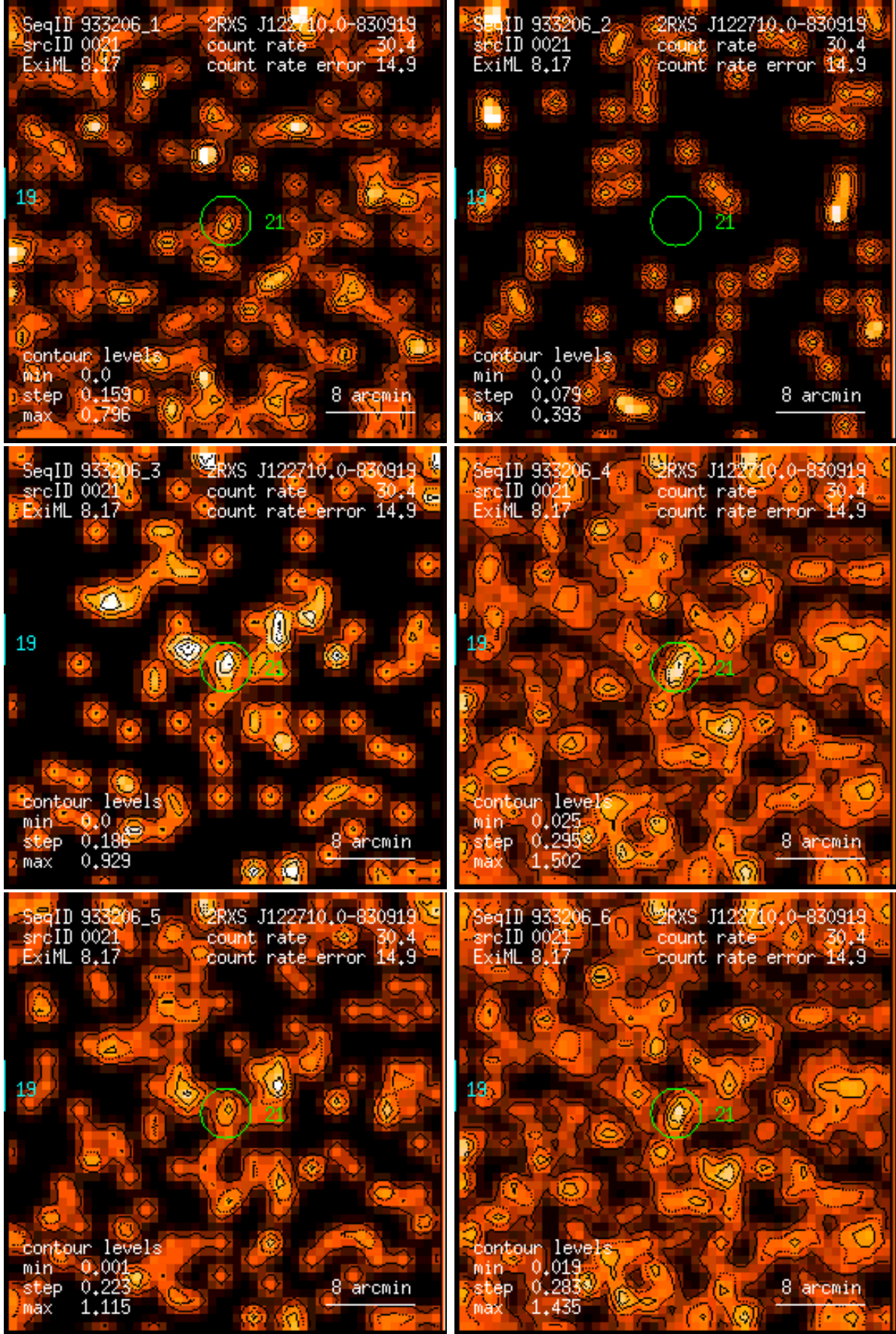
Figure 21: RASS 933206: detection 0021: band rate images, Gaussian filter: (1) PSPC channels 11 – 41, (2) 52 – 90, (3) 91 – 201, (4) 11 – 235, (5) 52 – 201, (6) 11 – 201. Broad band rates in counts/ks. Band rate contour levels in counts/ks/arcmin 2 .
