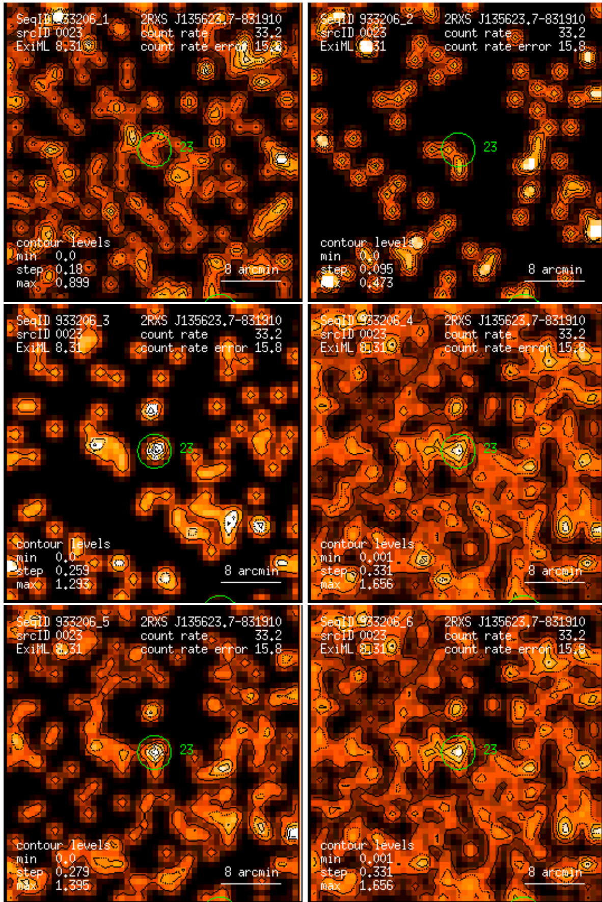
Figure 23: RASS 933206: detection 0023: band rate images, Gaussian filter: (1) PSPC channels 11 – 41, (2) 52 – 90, (3) 91 – 201, (4) 11 – 235, (5) 52 – 201, (6) 11 – 201. Broad band rates in counts/ks. Band rate contour levels in counts/ks/arcmin 2 .
