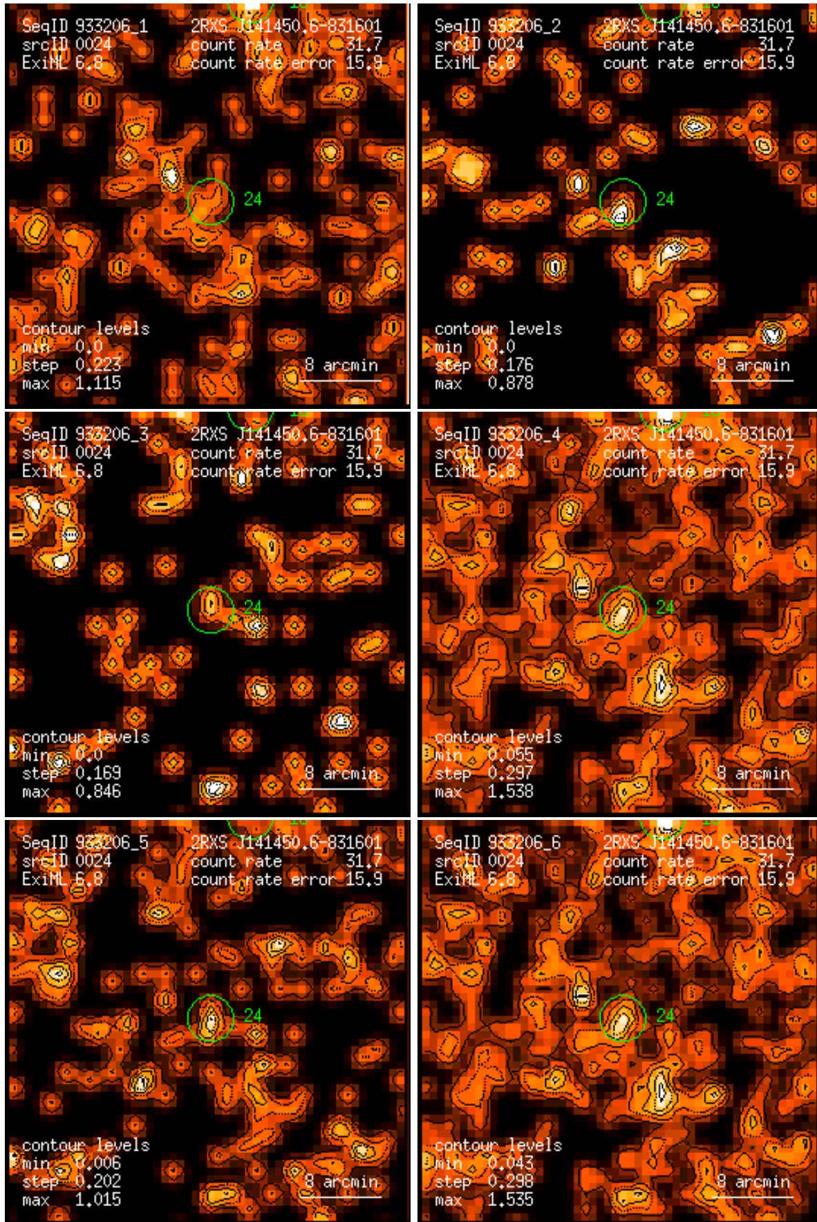
Figure 24: RASS 933206: detection 0024: band rate images, Gaussian filter: (1) PSPC channels 11 – 41, (2) 52 – 90, (3) 91 – 201, (4) 11 – 235, (5) 52 – 201, (6) 11 – 201. Broad band rates in counts/ks. Band rate contour levels in counts/ks/arcmin 2 .
