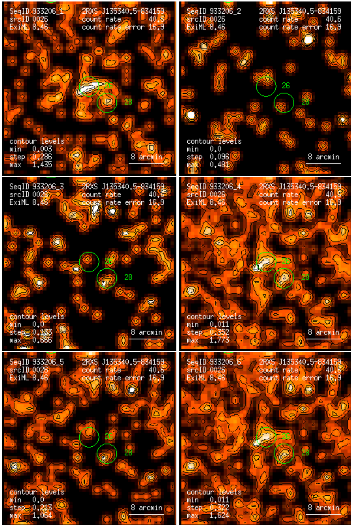
Figure 26: RASS 933206: detection 0026: band rate images, Gaussian filter: (1) PSPC channels 11 – 41, (2) 52 – 90, (3) 91 – 201, (4) 11 – 235, (5) 52 – 201, (6) 11 – 201. Broad band rates in counts/ks. Band rate contour levels in counts/ks/arcmin 2 .
