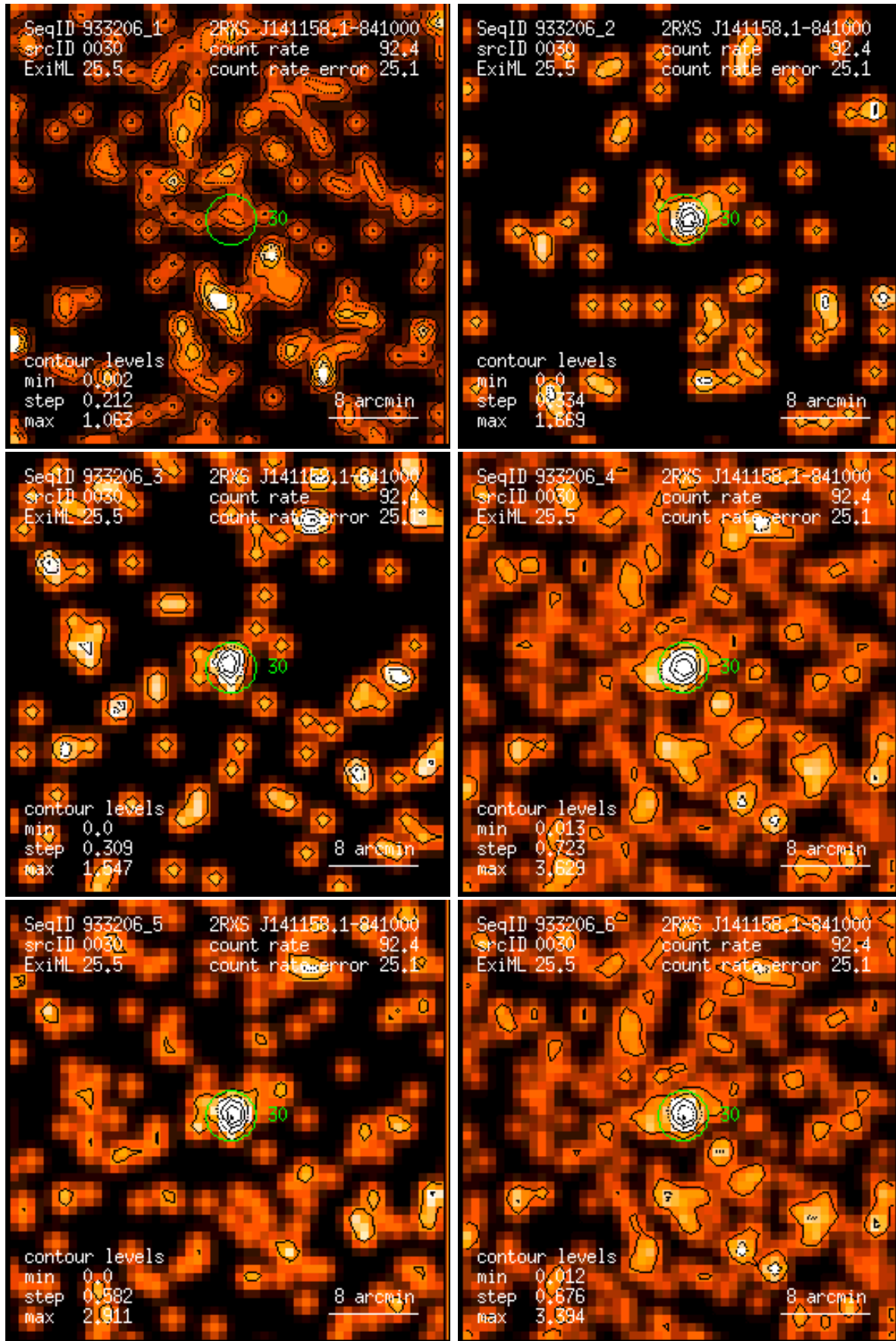
Figure 30: RASS 933206: detection 0030: band rate images, Gaussian filter: (1) PSPC channels 11 – 41, (2) 52 – 90, (3) 91 – 201, (4) 11 – 235, (5) 52 – 201, (6) 11 – 201. Broad band rates in counts/ks. Band rate contour levels in counts/ks/arcmin 2 .
