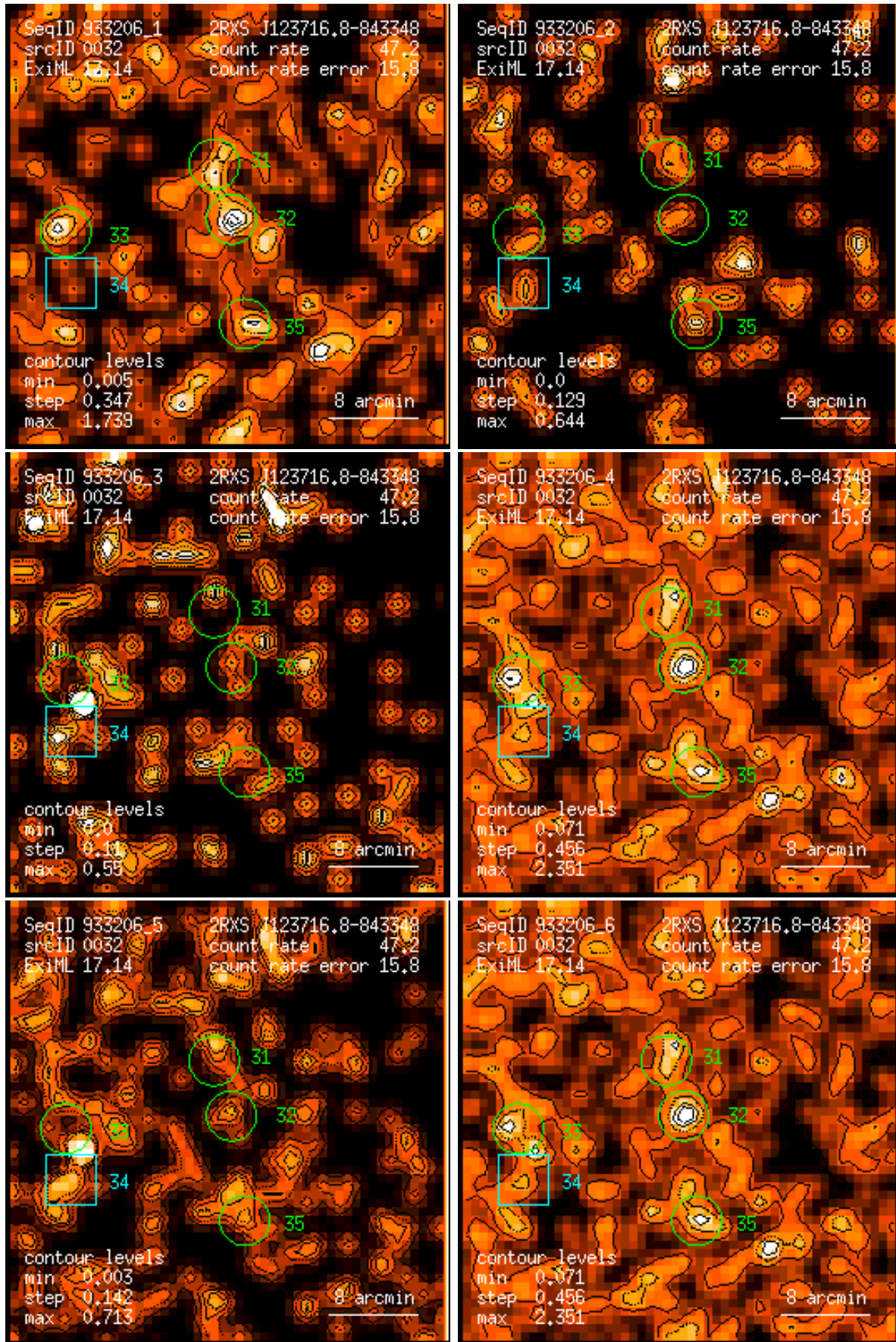
Figure 32: RASS 933206: detection 0032: band rate images, Gaussian filter: (1) PSPC channels 11 – 41, (2) 52 – 90, (3) 91 – 201, (4) 11 – 235, (5) 52 – 201, (6) 11 – 201. Broad band rates in counts/ks. Band rate contour levels in counts/ks/arcmin 2 .
