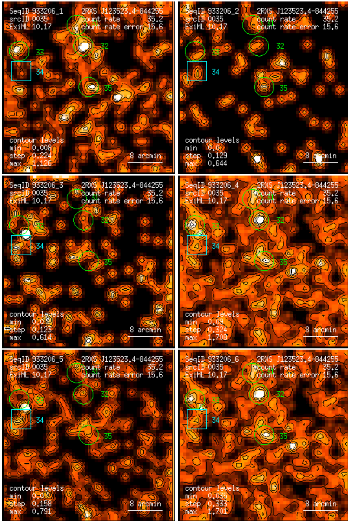
Figure 35: RASS 933206: detection 0035: band rate images, Gaussian filter: (1) PSPC channels 11 – 41, (2) 52 – 90, (3) 91 – 201, (4) 11 – 235, (5) 52 – 201, (6) 11 – 201. Broad band rates in counts/ks. Band rate contour levels in counts/ks/arcmin 2 .
