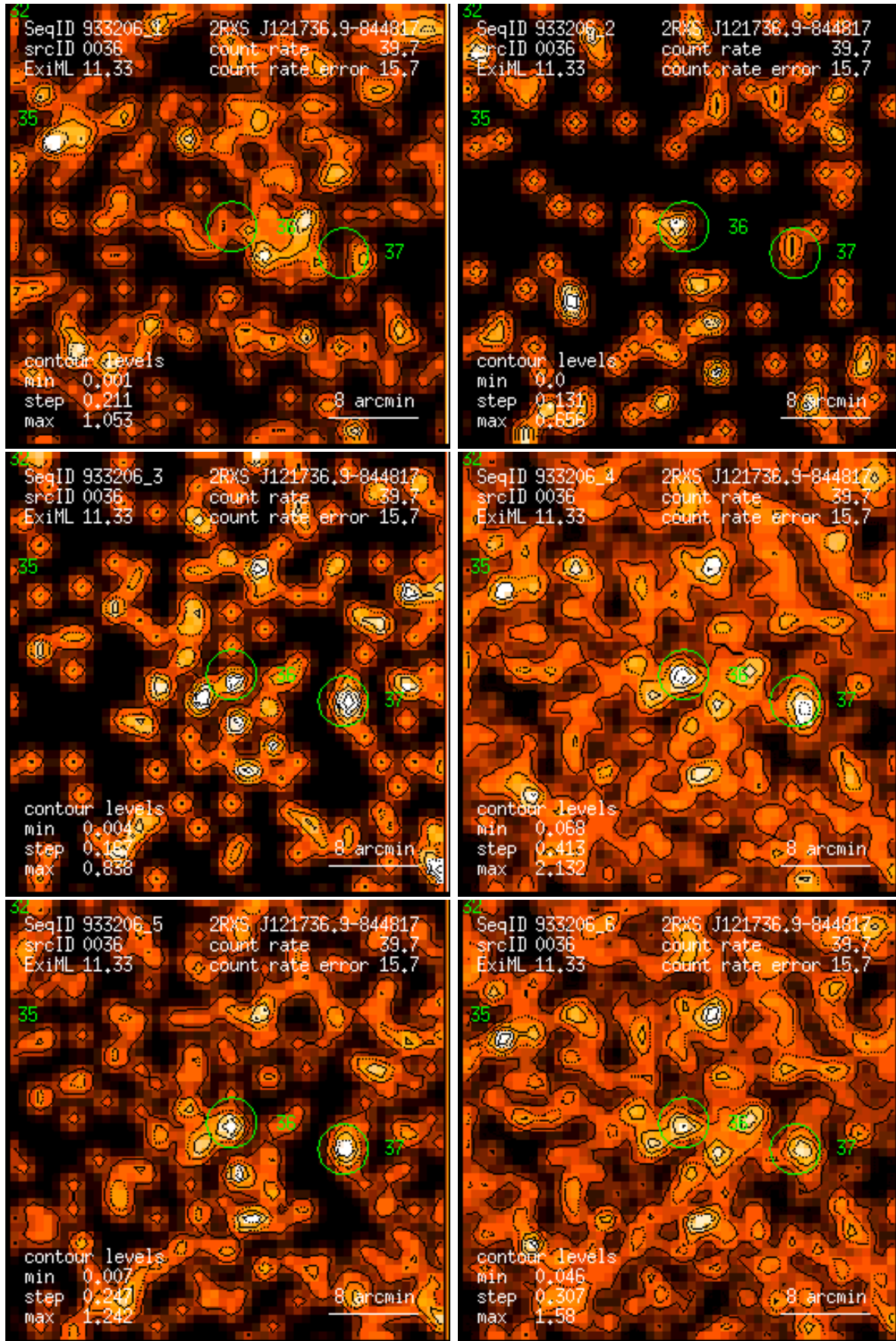
Figure 36: RASS 933206: detection 0036: band rate images, Gaussian filter: (1) PSPC channels 11 – 41, (2) 52 – 90, (3) 91 – 201, (4) 11 – 235, (5) 52 – 201, (6) 11 – 201. Broad band rates in counts/ks. Band rate contour levels in counts/ks/arcmin 2 .
