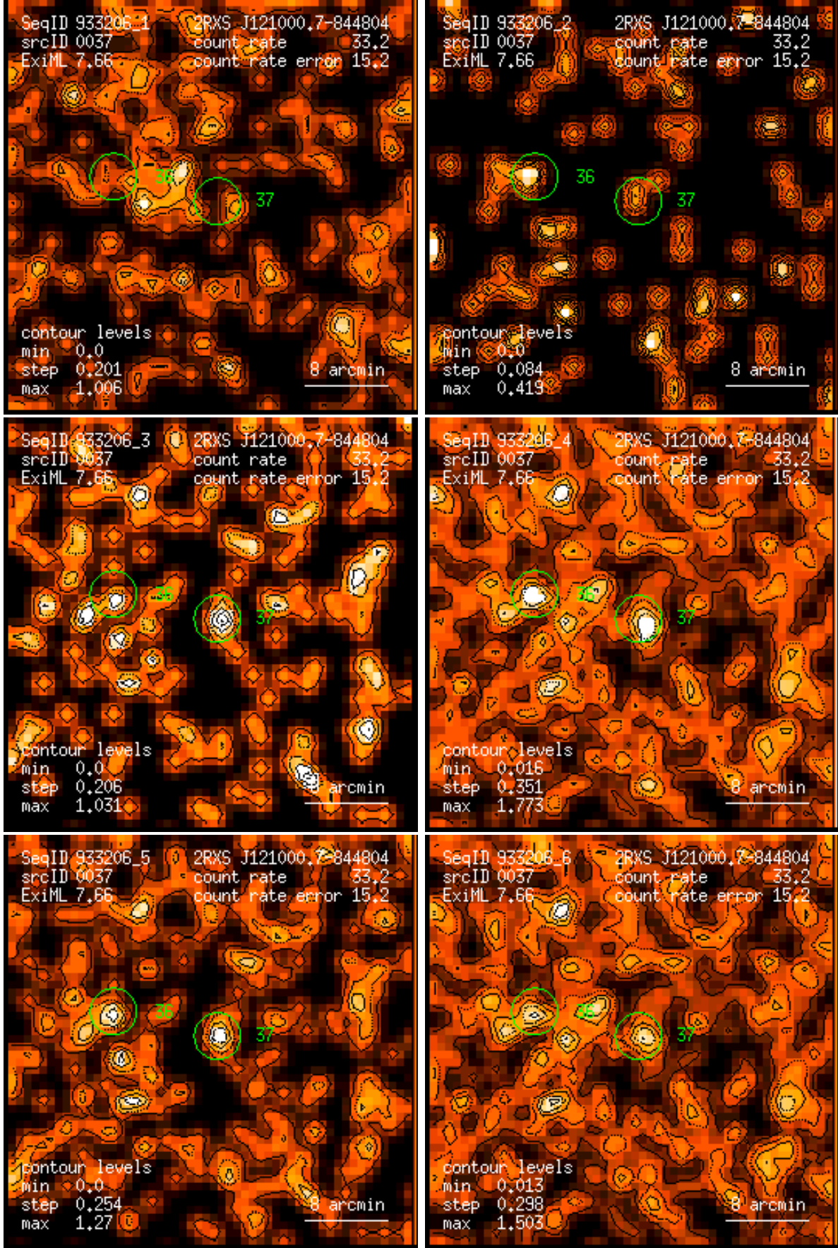
Figure 37: RASS 933206: detection 0037: band rate images, Gaussian filter: (1) PSPC channels 11 – 41, (2) 52 – 90, (3) 91 – 201, (4) 11 – 235, (5) 52 – 201, (6) 11 – 201. Broad band rates in counts/ks. Band rate contour levels in counts/ks/arcmin 2 .
