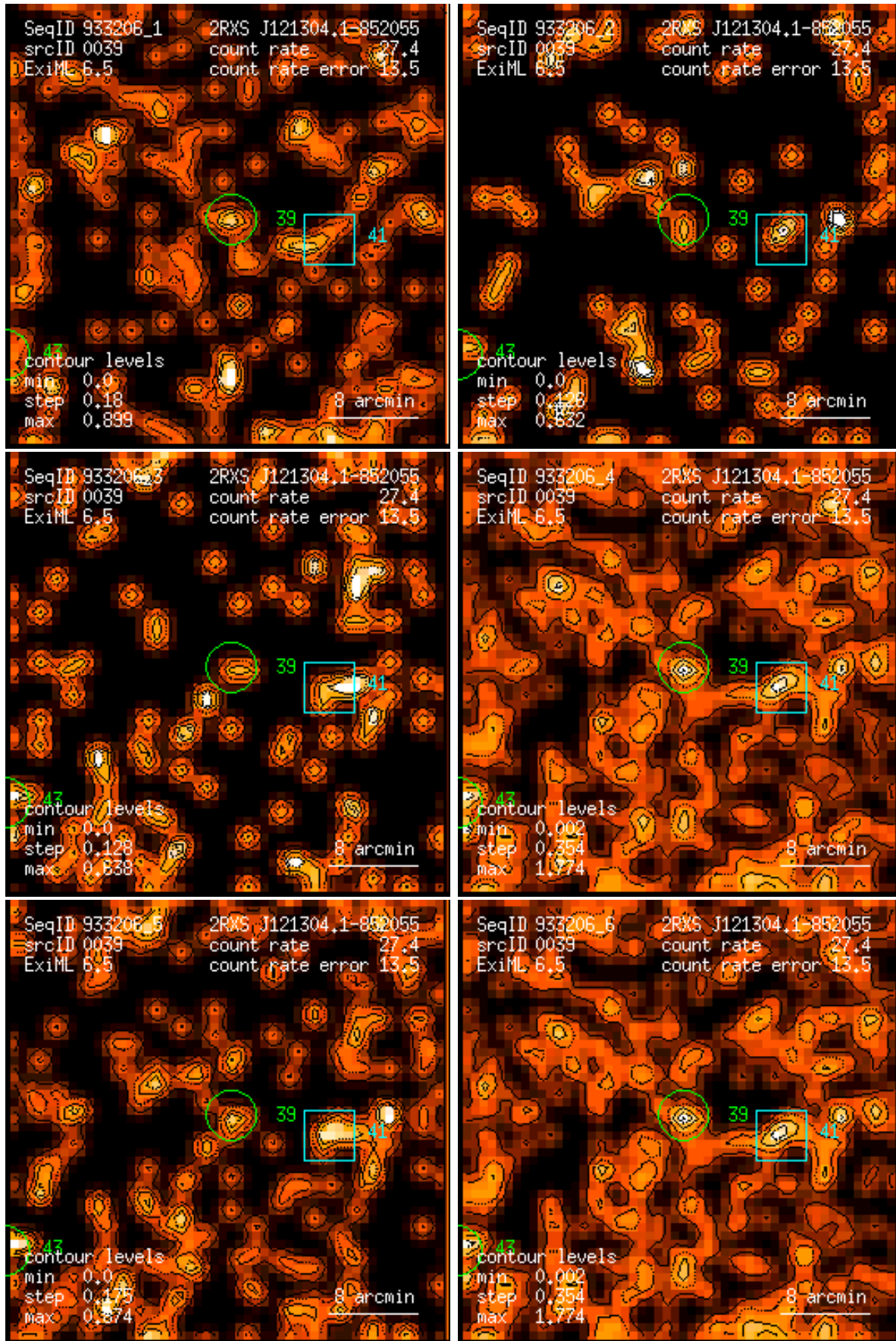
Figure 39: RASS 933206: detection 0039: band rate images, Gaussian filter: (1) PSPC channels 11 – 41, (2) 52 – 90, (3) 91 – 201, (4) 11 – 235, (5) 52 – 201, (6) 11 – 201. Broad band rates in counts/ks. Band rate contour levels in counts/ks/arcmin 2 .
