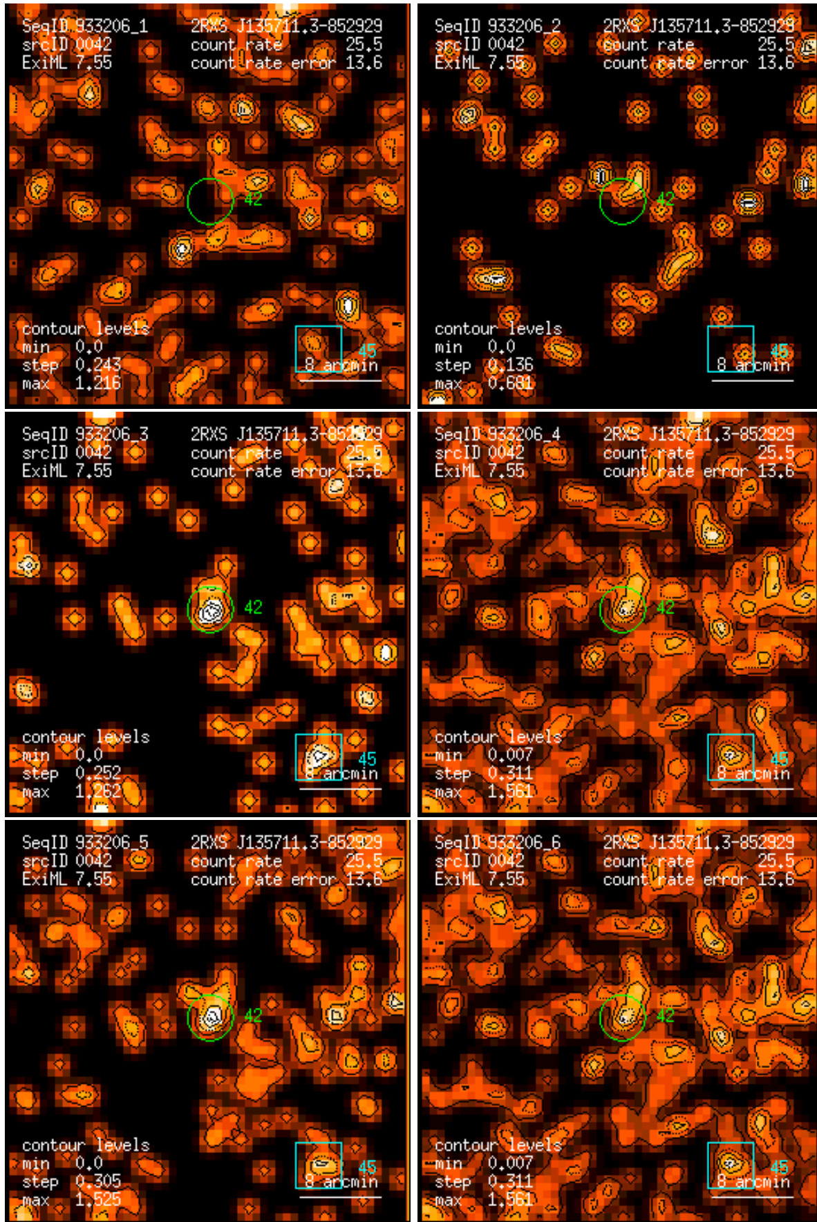
Figure 42: RASS 933206: detection 0042: band rate images, Gaussian filter: (1) PSPC channels 11 – 41, (2) 52 – 90, (3) 91 – 201, (4) 11 – 235, (5) 52 – 201, (6) 11 – 201. Broad band rates in counts/ks. Band rate contour levels in counts/ks/arcmin 2 .
