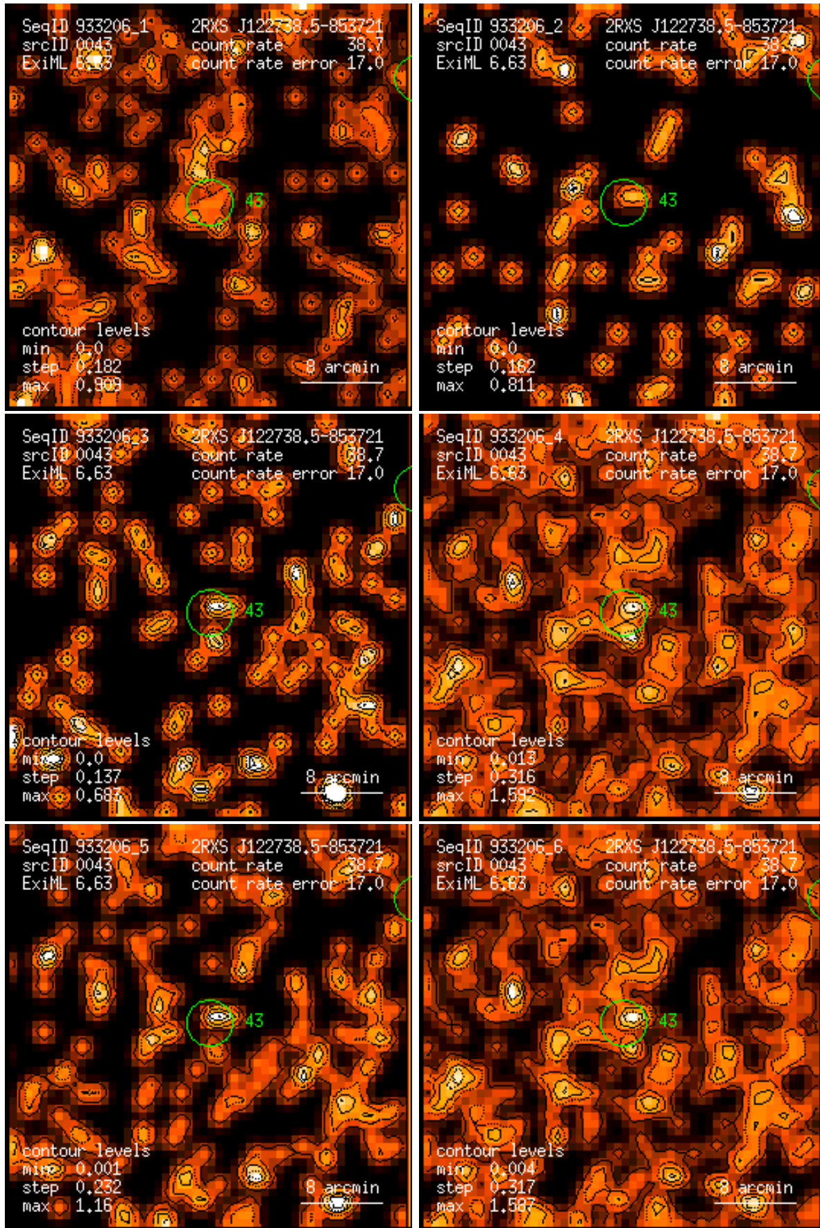
Figure 43: RASS 933206: detection 0043: band rate images, Gaussian filter: (1) PSPC channels 11 – 41, (2) 52 – 90, (3) 91 – 201, (4) 11 – 235, (5) 52 – 201, (6) 11 – 201. Broad band rates in counts/ks. Band rate contour levels in counts/ks/arcmin 2 .
