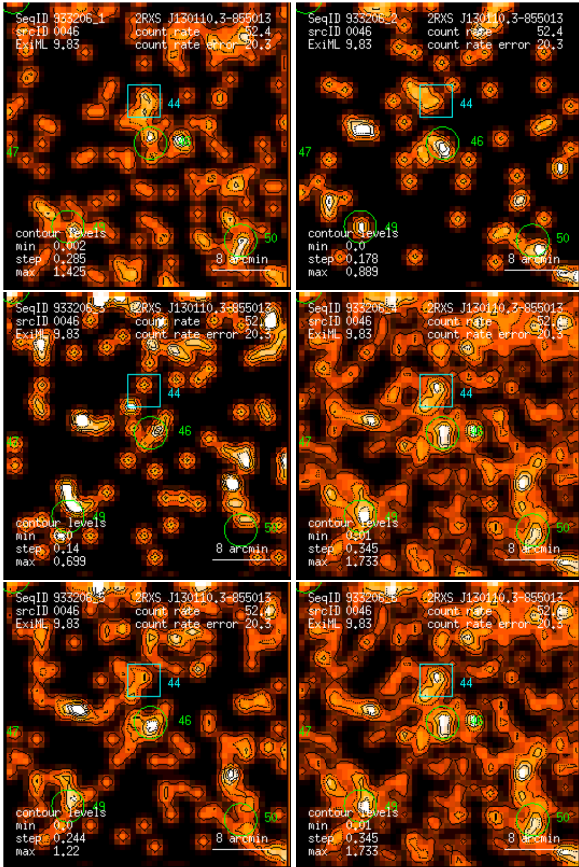
Figure 46: RASS 933206: detection 0046: band rate images, Gaussian filter: (1) PSPC channels 11 – 41, (2) 52 – 90, (3) 91 – 201, (4) 11 – 235, (5) 52 – 201, (6) 11 – 201. Broad band rates in counts/ks. Band rate contour levels in counts/ks/arcmin 2 .
