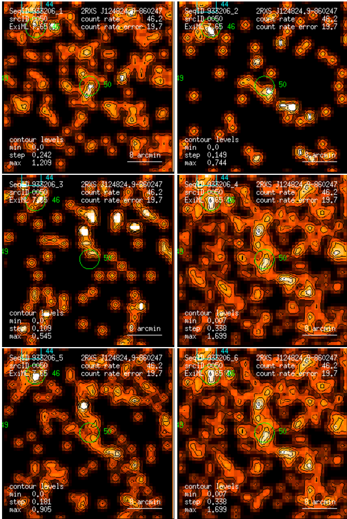
Figure 50: RASS 933206: detection 0050: band rate images, Gaussian filter: (1) PSPC channels 11 – 41, (2) 52 – 90, (3) 91 – 201, (4) 11 – 235, (5) 52 – 201, (6) 11 – 201. Broad band rates in counts/ks. Band rate contour levels in counts/ks/arcmin 2 .
