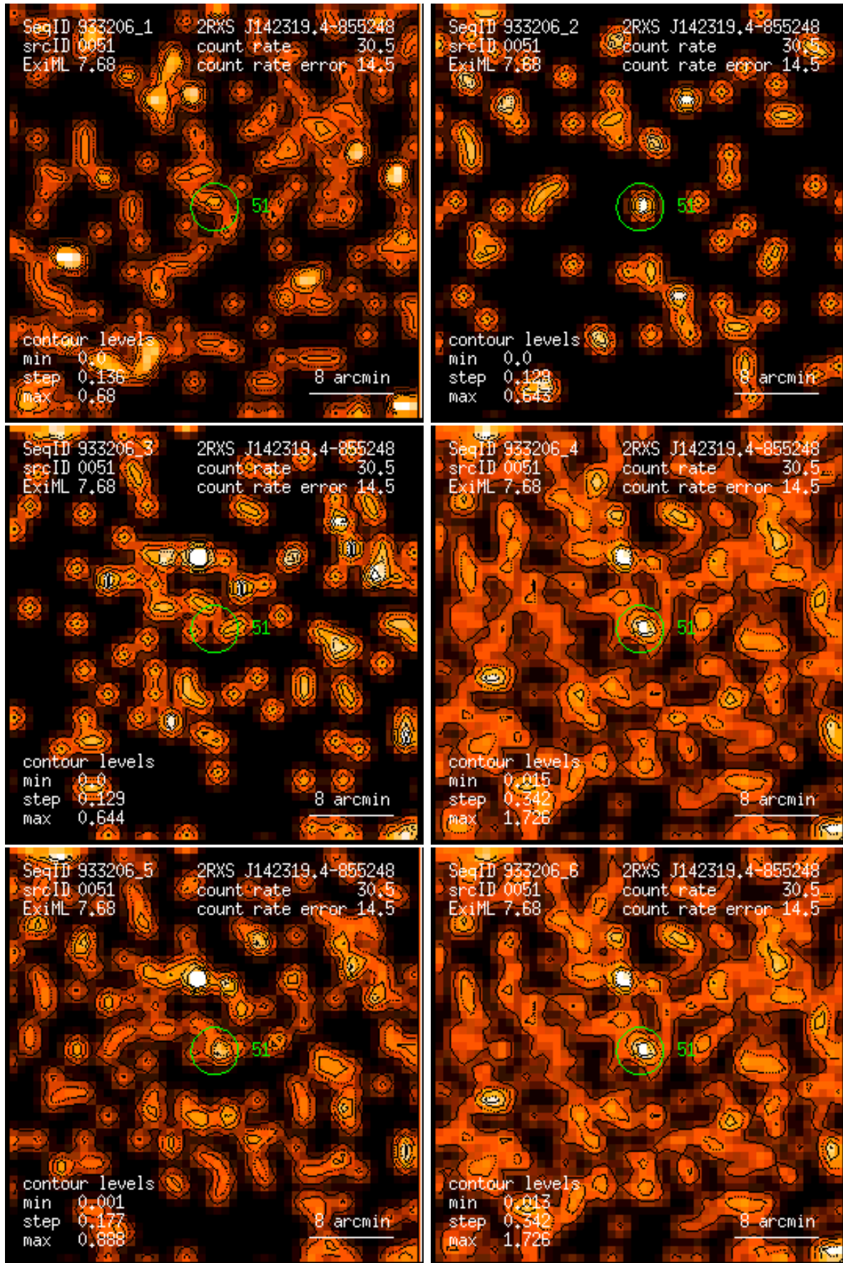
Figure 51: RASS 933206: detection 0051: band rate images, Gaussian filter: (1) PSPC channels 11 – 41, (2) 52 – 90, (3) 91 – 201, (4) 11 – 235, (5) 52 – 201, (6) 11 – 201. Broad band rates in counts/ks. Band rate contour levels in counts/ks/arcmin 2 .
