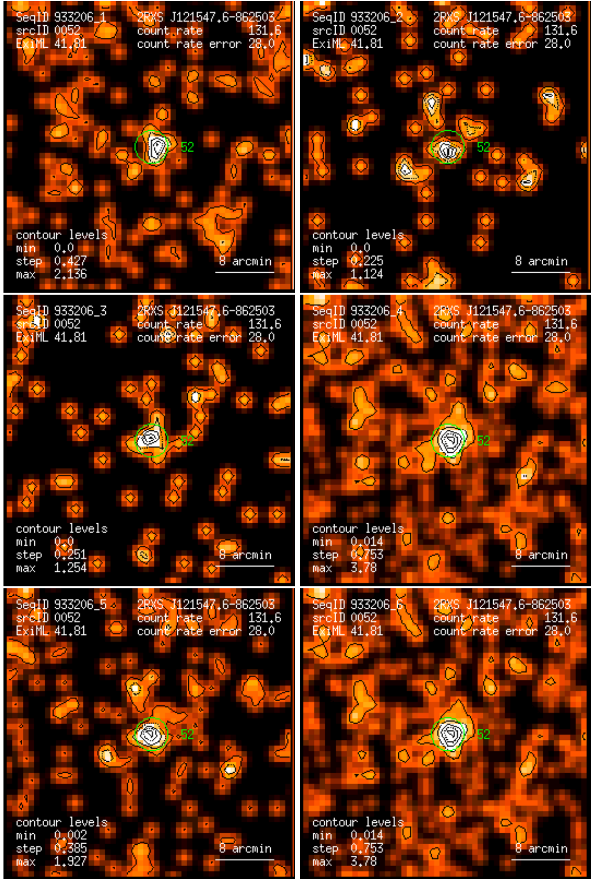
Figure 52: RASS 933206: detection 0052: band rate images, Gaussian filter: (1) PSPC channels 11 – 41, (2) 52 – 90, (3) 91 – 201, (4) 11 – 235, (5) 52 – 201, (6) 11 – 201. Broad band rates in counts/ks. Band rate contour levels in counts/ks/arcmin 2 .
