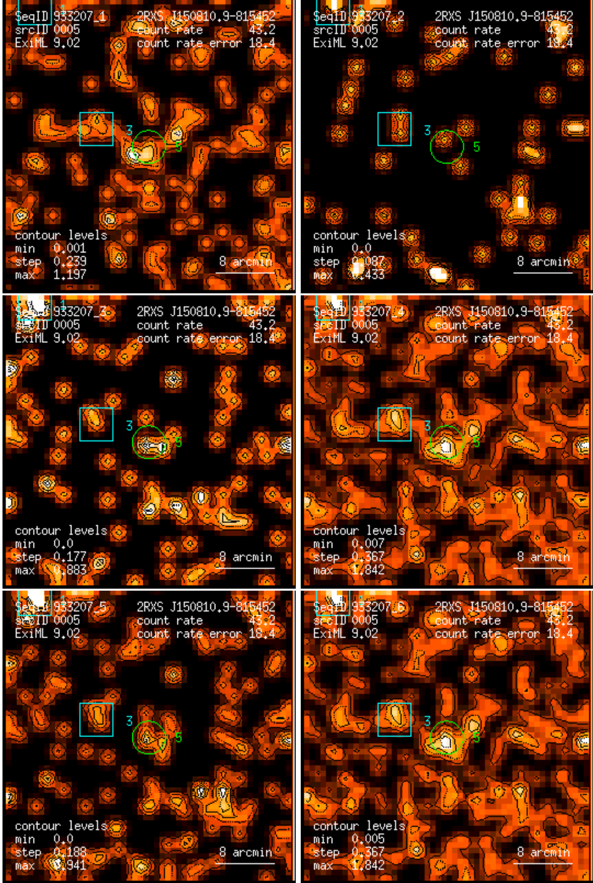
Figure 5: RASS 933207: detection 0005: band rate images, Gaussian filter: (1) PSPC channels 11 – 41, (2) 52 – 90, (3) 91 – 201, (4) 11 – 235, (5) 52 – 201, (6) 11 – 201. Broad band rates in counts/ks. Band rate contour levels in counts/ks/arcmin 2 .
