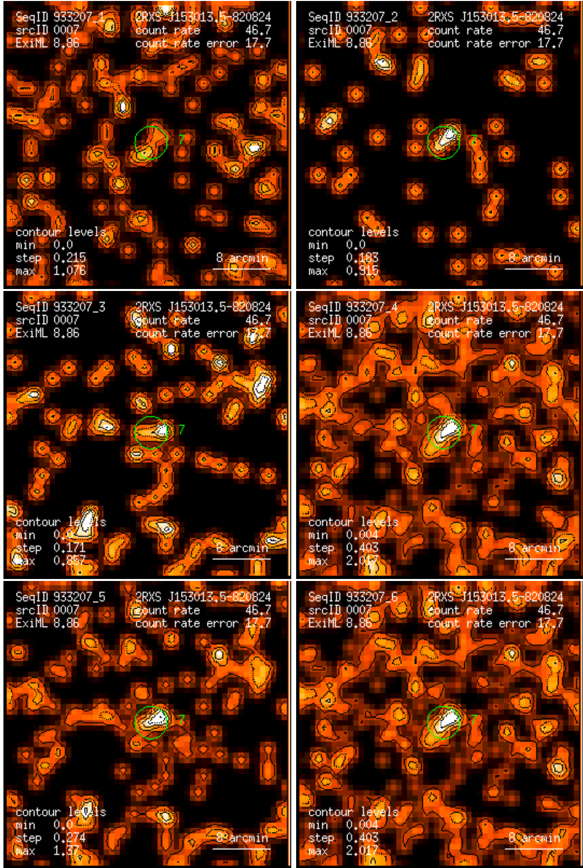
Figure 7: RASS 933207: detection 0007: band rate images, Gaussian filter: (1) PSPC channels 11 – 41, (2) 52 – 90, (3) 91 – 201, (4) 11 – 235, (5) 52 – 201, (6) 11 – 201. Broad band rates in counts/ks. Band rate contour levels in counts/ks/arcmin 2 .
