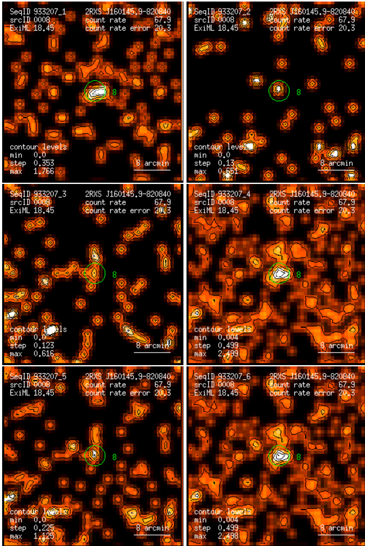
Figure 8: RASS 933207: detection 0008: band rate images, Gaussian filter: (1) PSPC channels 11 – 41, (2) 52 – 90, (3) 91 – 201, (4) 11 – 235, (5) 52 – 201, (6) 11 – 201. Broad band rates in counts/ks. Band rate contour levels in counts/ks/arcmin 2 .
