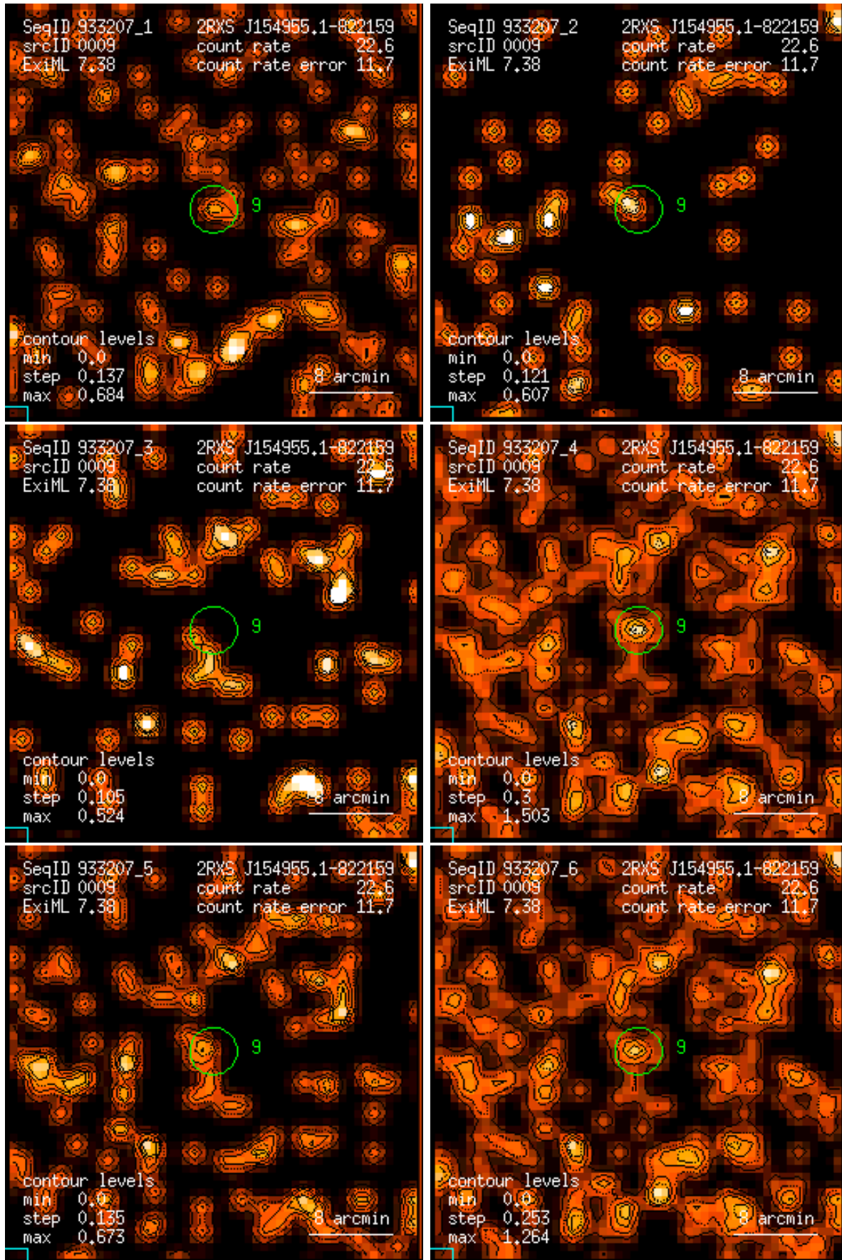
Figure 9: RASS 933207: detection 0009: band rate images, Gaussian filter: (1) PSPC channels 11 – 41, (2) 52 – 90, (3) 91 – 201, (4) 11 – 235, (5) 52 – 201, (6) 11 – 201. Broad band rates in counts/ks. Band rate contour levels in counts/ks/arcmin 2 .
