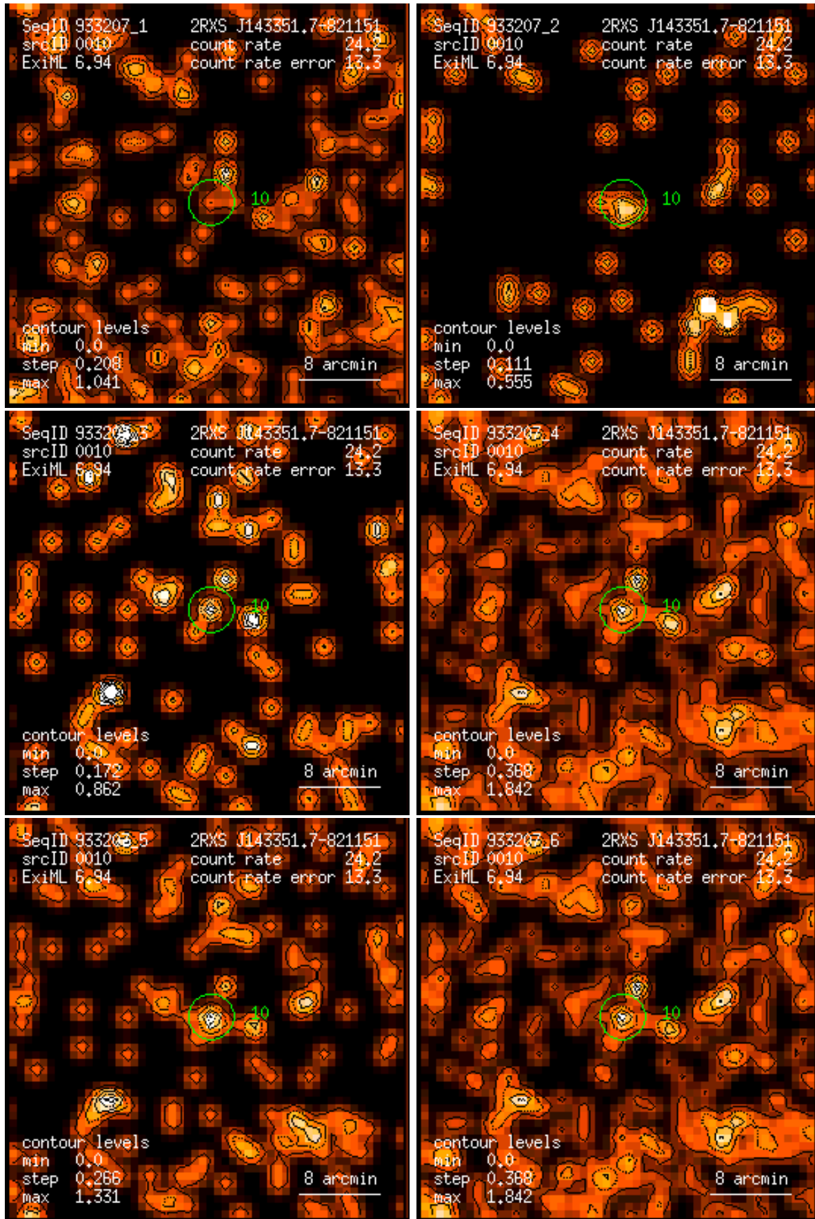
Figure 10: RASS 933207: detection 0010: band rate images, Gaussian filter: (1) PSPC channels 11 – 41, (2) 52 – 90, (3) 91 – 201, (4) 11 – 235, (5) 52 – 201, (6) 11 – 201. Broad band rates in counts/ks. Band rate contour levels in counts/ks/arcmin 2 .
