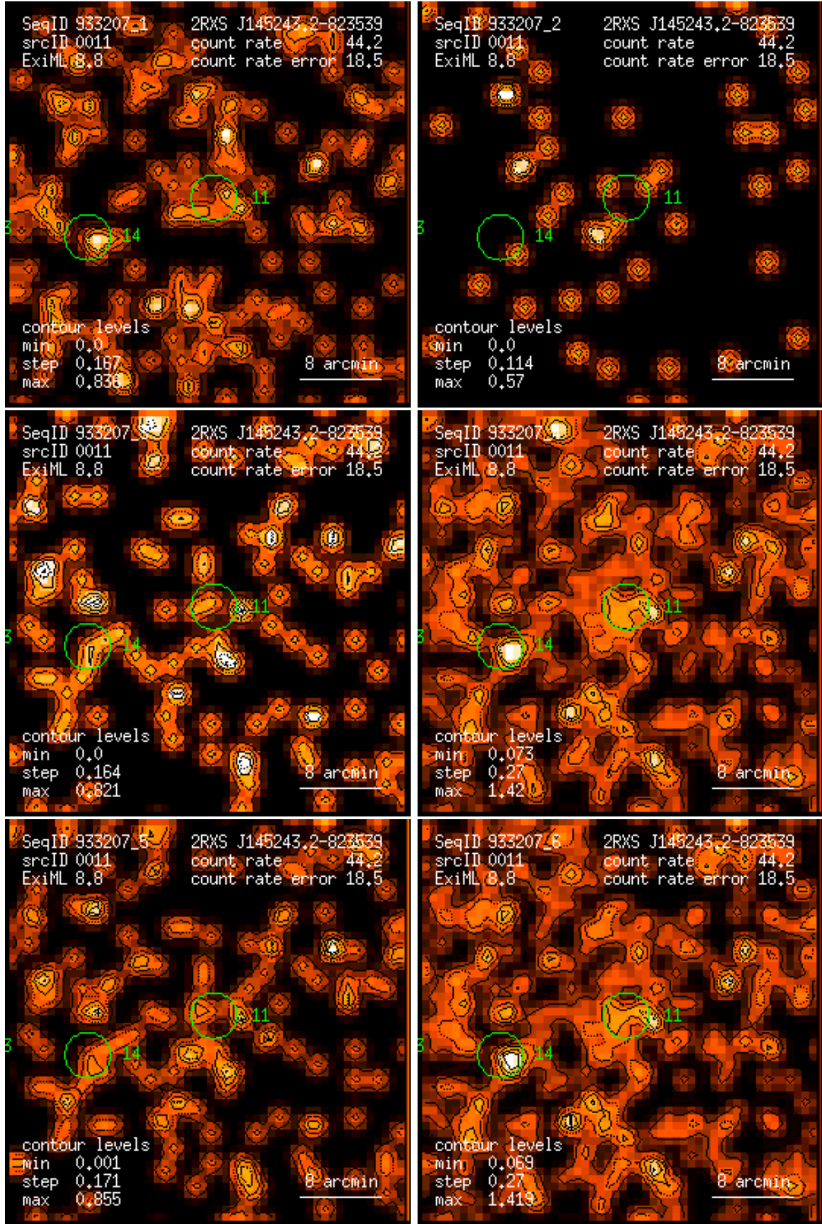
Figure 11: RASS 933207: detection 0011: band rate images, Gaussian filter: (1) PSPC channels 11 – 41, (2) 52 – 90, (3) 91 – 201, (4) 11 – 235, (5) 52 – 201, (6) 11 – 201. Broad band rates in counts/ks. Band rate contour levels in counts/ks/arcmin 2 .
