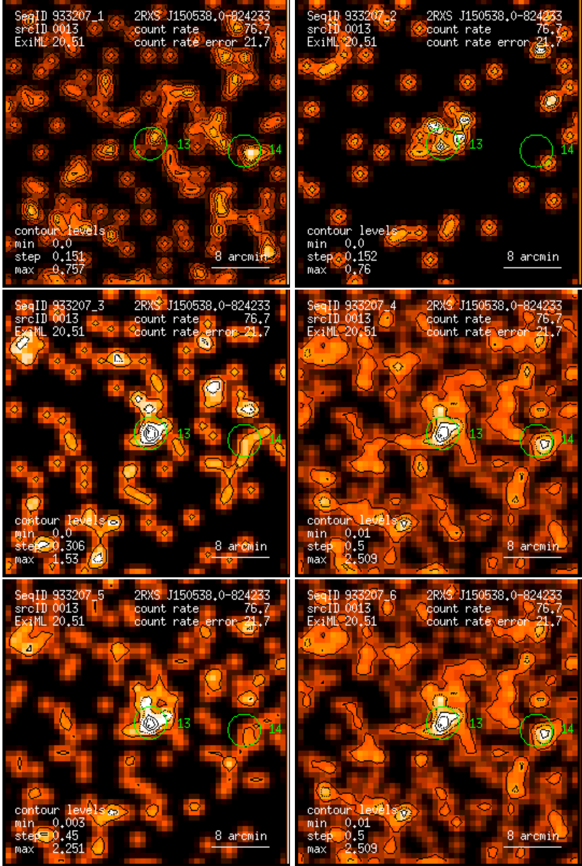
Figure 13: RASS 933207: detection 0013: band rate images, Gaussian filter: (1) PSPP channels 11 – 41, (2) 52 – 90, (3) 91 – 201, (4) 11 – 235, (5) 52 – 201, (6) 11 – 201. Broad band rates in counts/ks. Band rate contour levels in counts/ks/arcmin 2 .
