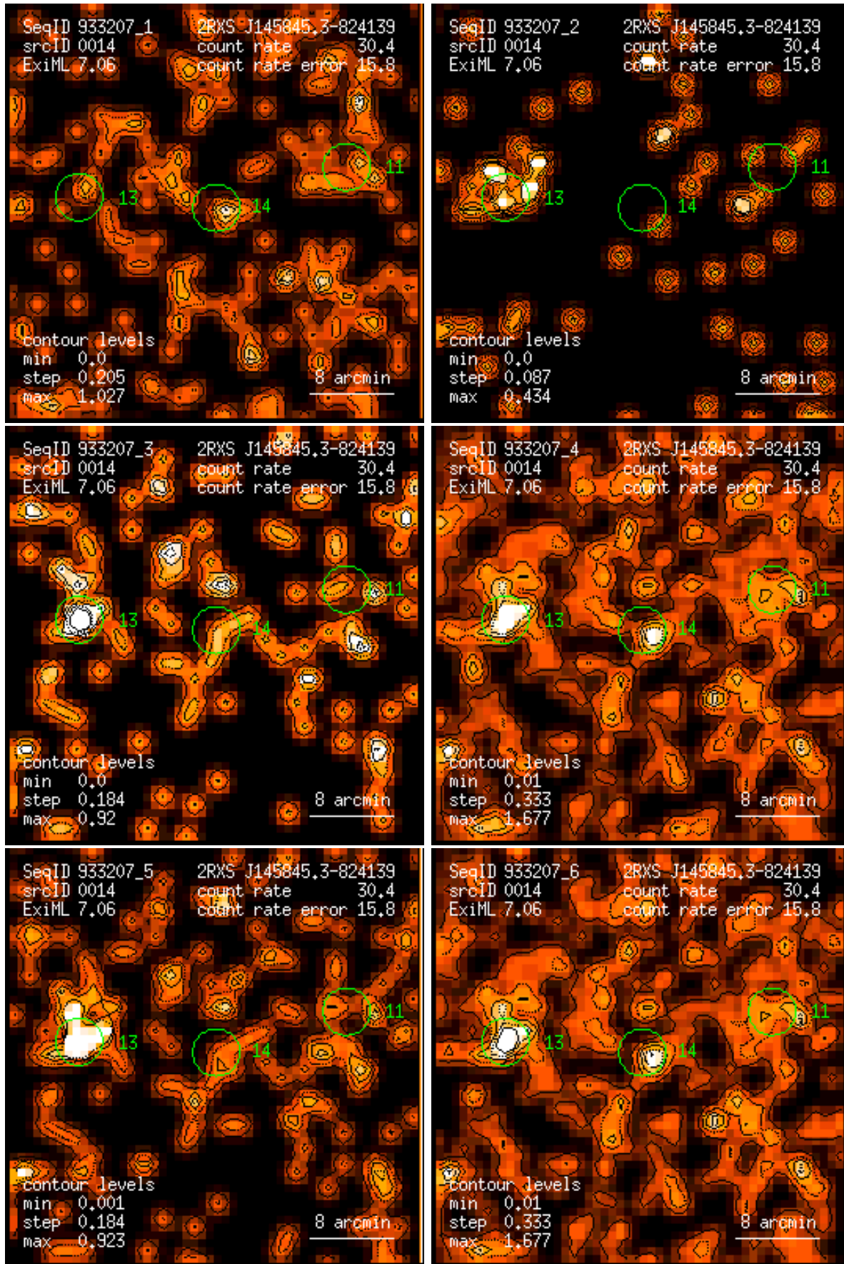
Figure 14: RASS 933207: detection 0014: band rate images, Gaussian filter: (1) PSPC channels 11 – 41, (2) 52 – 90, (3) 91 – 201, (4) 11 – 235, (5) 52 – 201, (6) 11 – 201. Broad band rates in counts/ks. Band rate contour levels in counts/ks/arcmin 2 .
