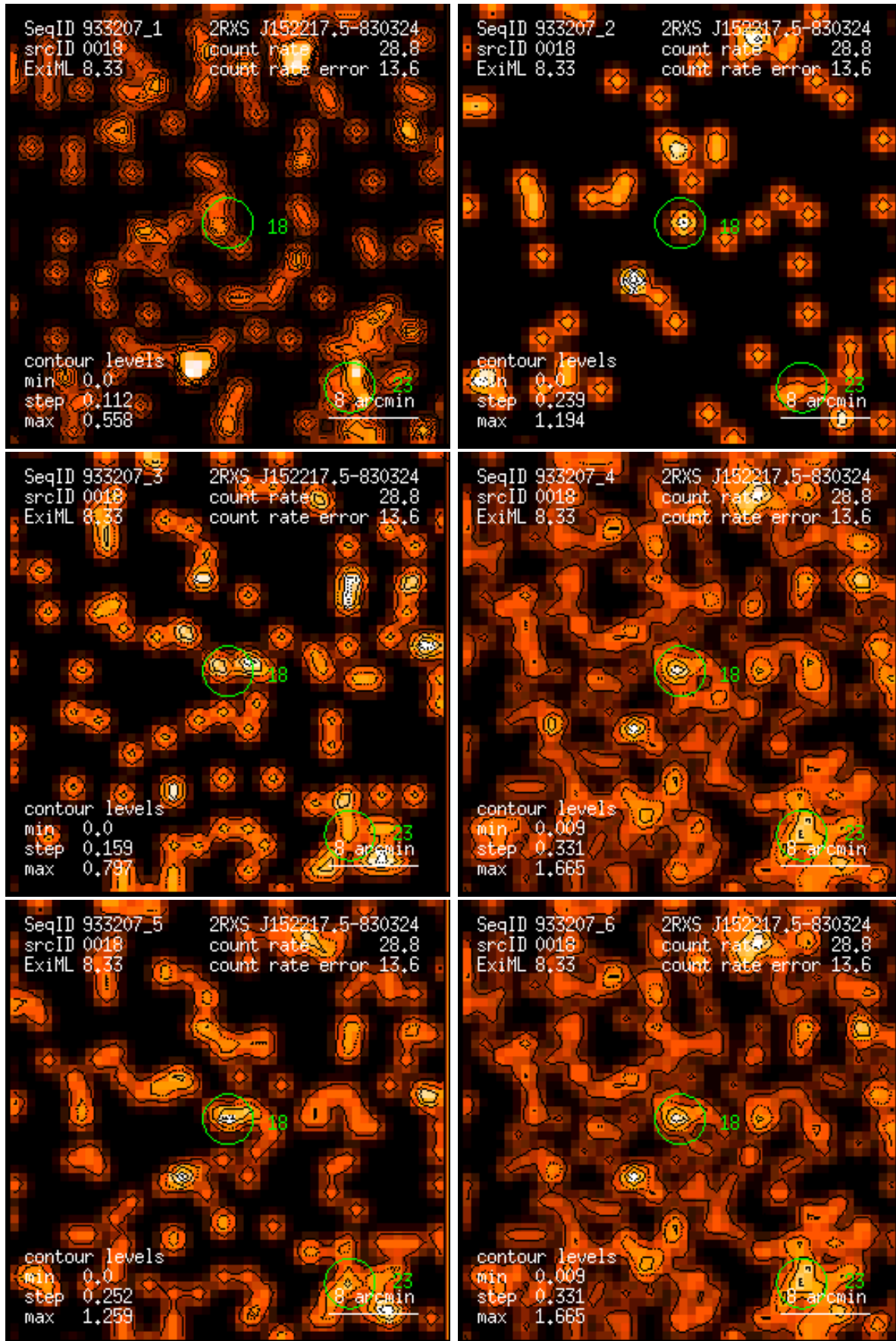
Figure 18: RASS 933207: detection 0018: band rate images, Gaussian filter: (1) PSPC channels 11 – 41, (2) 52 – 90, (3) 91 – 201, (4) 11 – 235, (5) 52 – 201, (6) 11 – 201. Broad band rates in counts/ks. Band rate contour levels in counts/ks/arcmin 2 .
