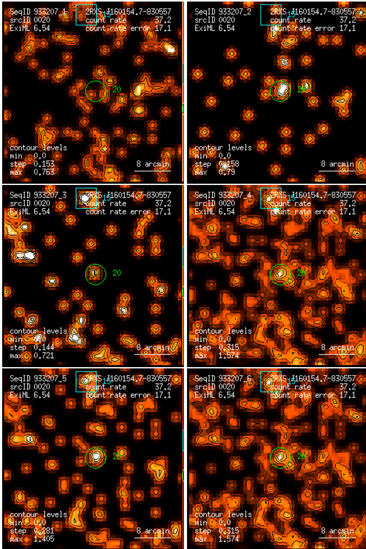
Figure 20: RASS 933207: detection 0020: band rate images, Gaussian filter: (1) PSPC channels 11 – 41, (2) 52 – 90, (3) 91 – 201, (4) 11 – 235, (5) 52 – 201, (6) 11 – 201. Broad band rates in counts/ks. Band rate contour levels in counts/ks/arcmin 2 .
