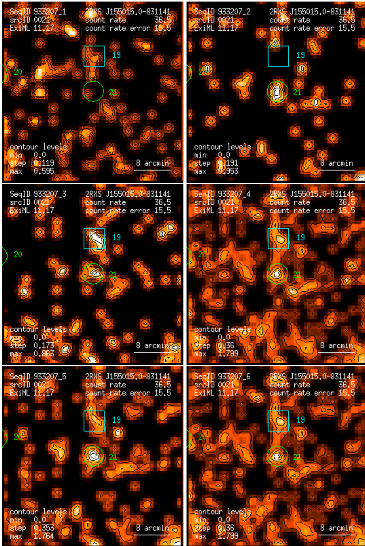
Figure 21: RASS 933207: detection 0021: band rate images, Gaussian filter: (1) PSPC channels 11 – 41, (2) 52 – 90, (3) 91 – 201, (4) 11 – 235, (5) 52 – 201, (6) 11 – 201. Broad band rates in counts/ks. Band rate contour levels in counts/ks/arcmin 2 .
