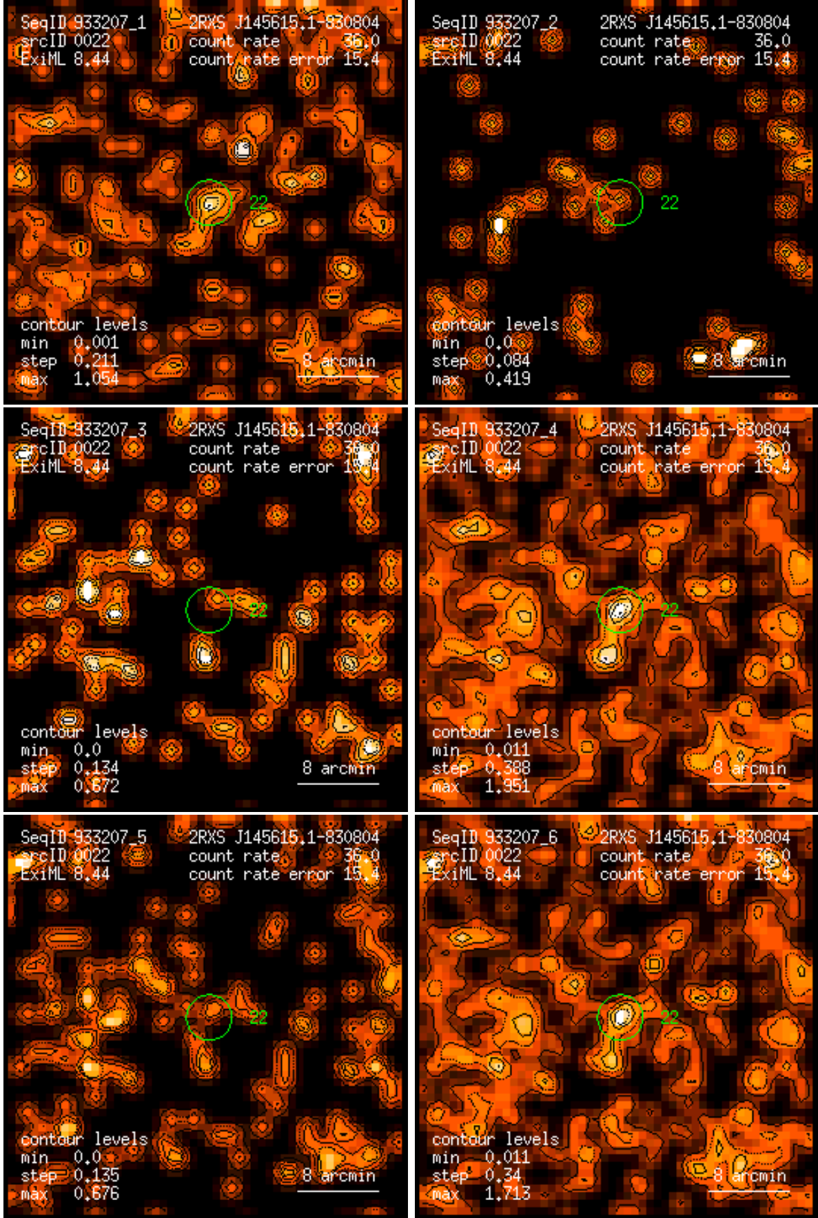
Figure 22: RASS 933207: detection 0022: band rate images, Gaussian filter: (1) PSPC channels 11 – 41, (2) 52 – 90, (3) 91 – 201, (4) 11 – 235, (5) 52 – 201, (6) 11 – 201. Broad band rates in counts/ks. Band rate contour levels in counts/ks/arcmin 2 .
