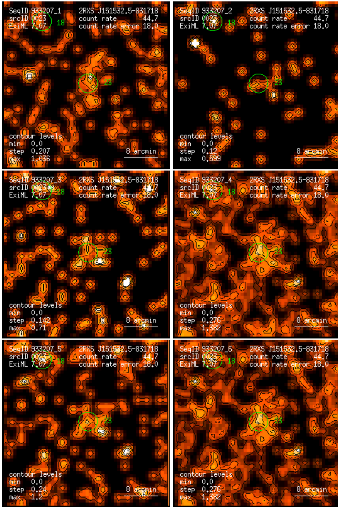
Figure 23: RASS 933207: detection 0023: band rate images, Gaussian filter: (1) PSPC channels 11 – 41, (2) 52 – 90, (3) 91 – 201, (4) 11 – 235, (5) 52 – 201, (6) 11 – 201. Broad band rates in counts/ks. Band rate contour levels in counts/ks/arcmin 2 .
