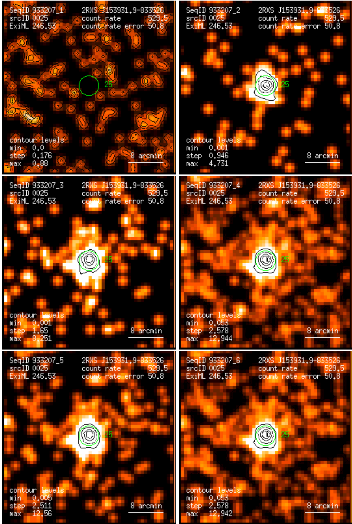
Figure 25: RASS 933207: detection 0025: band rate images, Gaussian filter: (1) PSPC channels 11 – 41, (2) 52 – 90, (3) 91 – 201, (4) 11 – 235, (5) 52 – 201, (6) 11 – 201. Broad band rates in counts/ks. Band rate contour levels in counts/ks/arcmin 2 .
