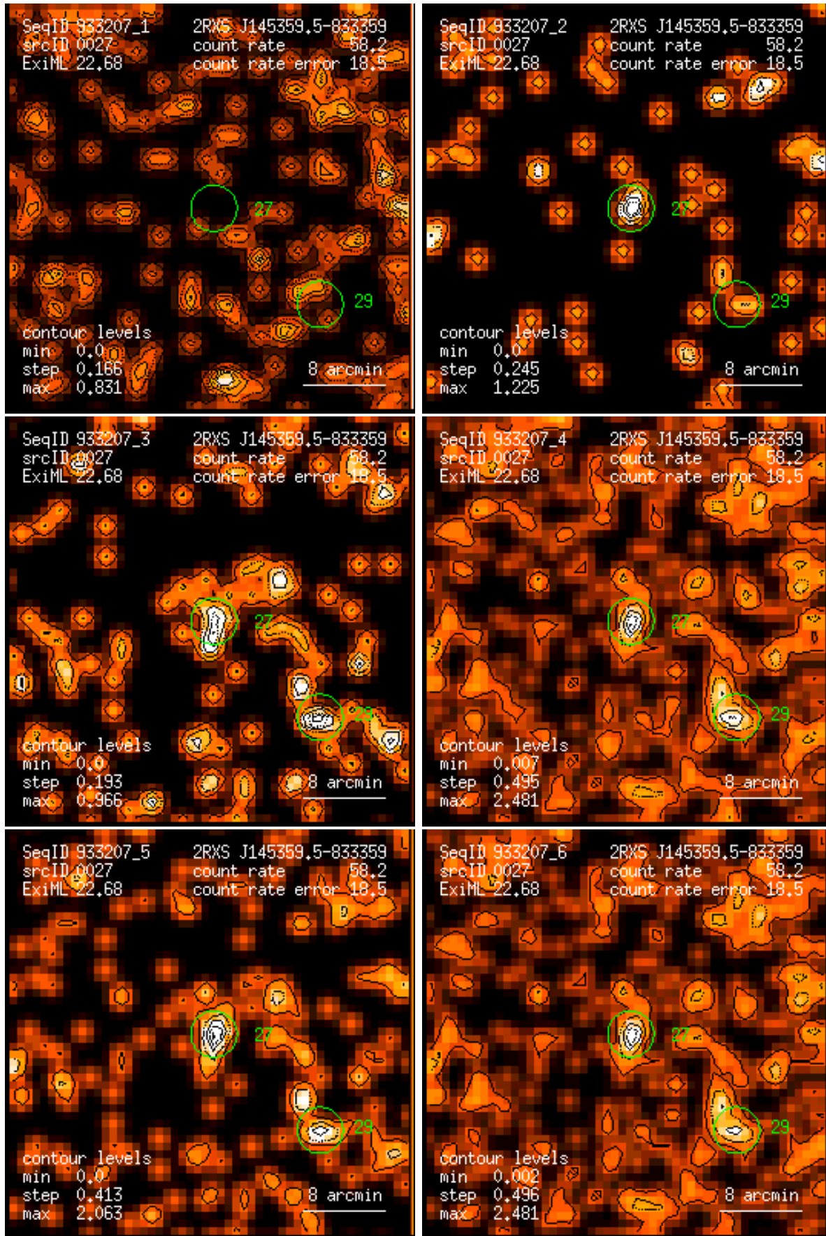
Figure 27: RASS 933207: detection 0027: band rate images, Gaussian filter: (1) PSPC channels 11 – 41, (2) 52 – 90, (3) 91 – 201, (4) 11 – 235, (5) 52 – 201, (6) 11 – 201. Broad band rates in counts/ks. Band rate contour levels in counts/ks/arcmin 2 .
