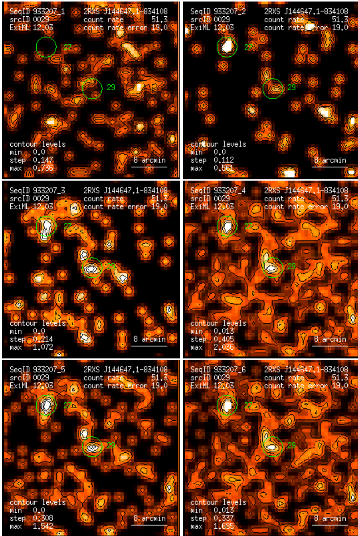
Figure 29: RASS 933207: detection 0029: band rate images, Gaussian filter: (1) PSPC channels 11 – 41, (2) 52 – 90, (3) 91 – 201, (4) 11 – 235, (5) 52 – 201, (6) 11 – 201. Broad band rates in counts/ks. Band rate contour levels in counts/ks/arcmin 2 .
