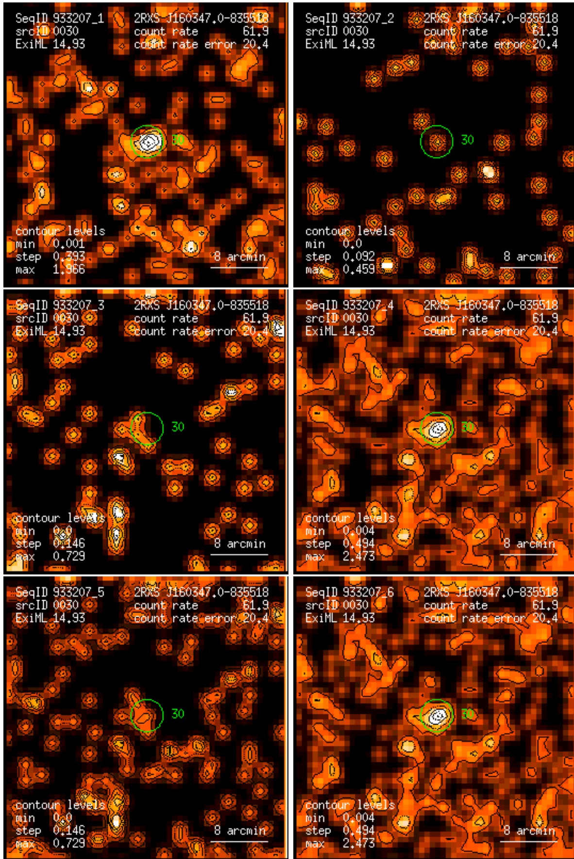
Figure 30: RASS 933207: detection 0030: band rate images, Gaussian filter: (1) PSPC channels 11 – 41, (2) 52 – 90, (3) 91 – 201, (4) 11 – 235, (5) 52 – 201, (6) 11 – 201. Broad band rates in counts/ks. Band rate contour levels in counts/ks/arcmin 2 .
