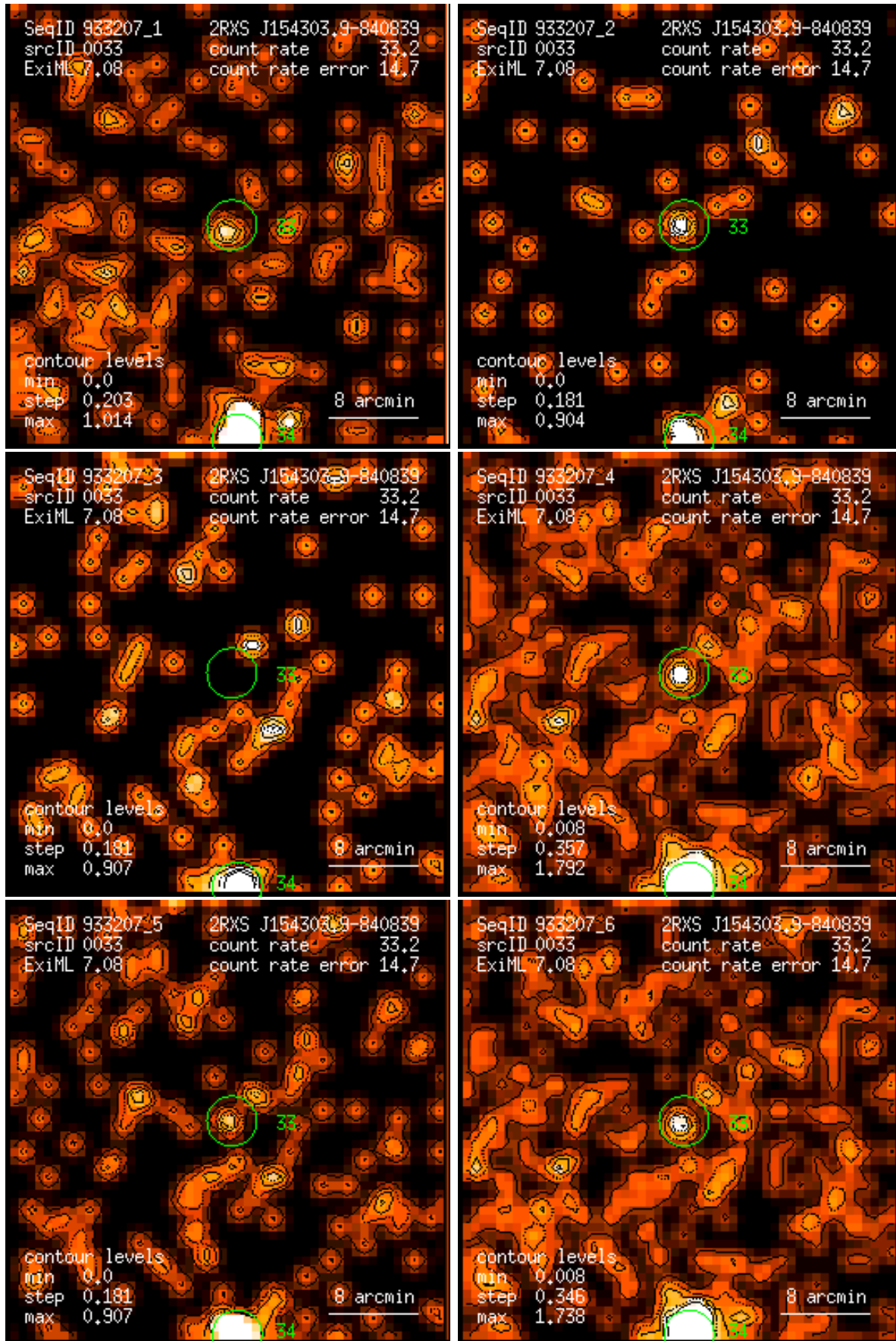
Figure 33: RASS 933207: detection 0033: band rate images, Gaussian filter: (1) PSPC channels 11 – 41, (2) 52 – 90, (3) 91 – 201, (4) 11 – 235, (5) 52 – 201, (6) 11 – 201. Broad band rates in counts/ks. Band rate contour levels in counts/ks/arcmin 2 .
